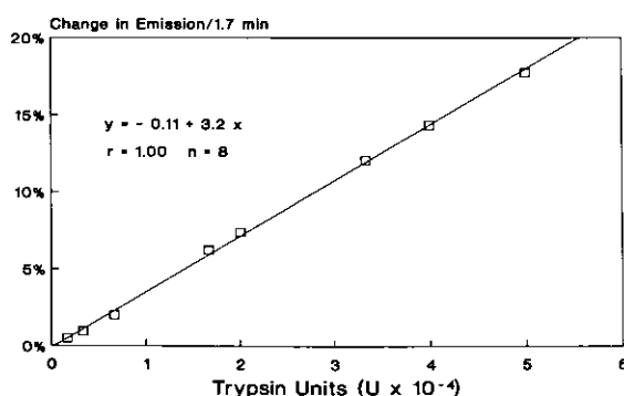
Fig. 4. Trypsin standard curve using different amounts of trypsin standard solution, expressed in units (U). The curve was fitted by linear regression. Substrate CBZ-L-Arg-MCA, 0.20 mMol in TRIS-HCl buffer, pH 8.0, 25°C, \delta t = 1.7 min., excitation 380 nm, emission 440 nm
