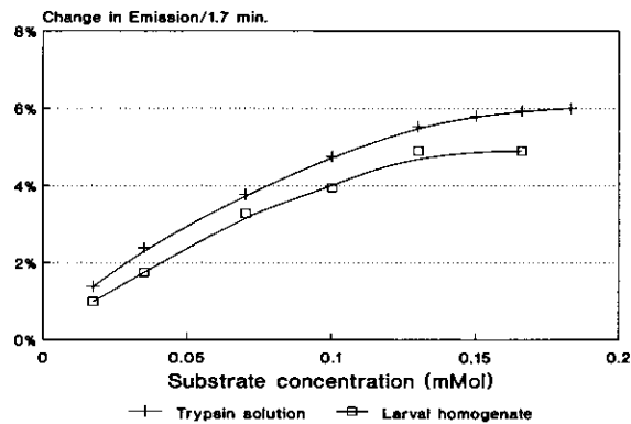
Fig. 2. Increase in emission in relation to the substrate concentration (abscissa gives the final concentrations) with a trypsin standard solution and with larval homogenate. Substrate CBZ-L-Arg-MCA in TRIS-HCl buffer, pH 8.0, 25 °C, excitation 380 nm, emission 440 nm, \delta t = 1.7 min.
