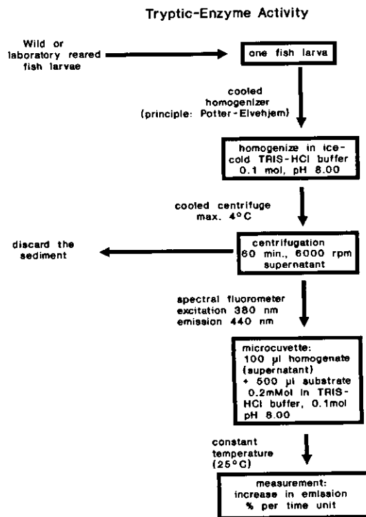
Fig. 1. Flow chart of analytical procedure
