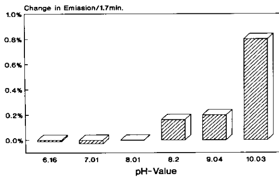
Fig. 6. Rates of non-enzymatic hydrolysis of the substrate CBZ-L-Arg-MCA, 0.20 mMol in TRIS-HCl buffer in relation to different pH-values in the assay solution, TRIS buffer 0.1 Mol, 25 ^{\circ} C, \delta t = 1.7 min., excitation 380 nm, emission 440 nm
