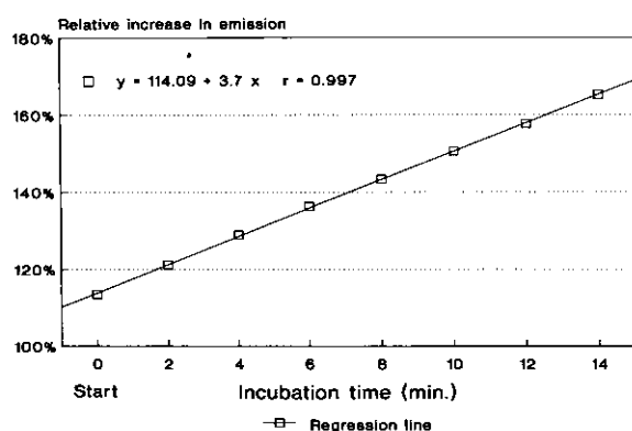
Fig. 3. Relative increase in emission during a total measuring period of 15 min., larval homogenate. The curve was fitted by linear regression. Substrate CBZ-L-Arg-MCA, 0.20 mMol in TRIS-HCl buffer, pH 8.0, 25°C, excitation 380 nm, emission 440 nm
