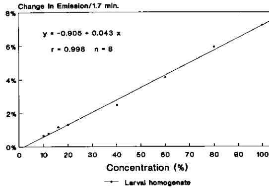
Fig. 5. Relationship between change in emission per time unit and the amount of larval homogenate. 100 % concentration means 100 \mu l undiluted larval homogenate in the assay solution. The curve was fitted by linear regression. Substrate CBZ-L-Arg-MCA, 0.20 mMol in TRIS-HCl buffer, pH 8.0, 25 ^{\circ} C, \delta t = 1.7 min., excitation 380 nm, emission 440 nm
