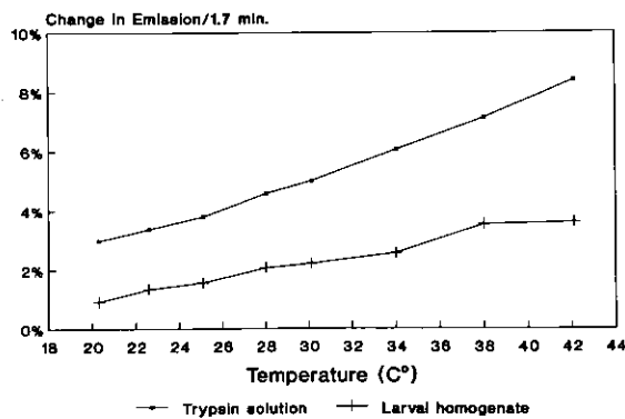
Fig. 7. Change in emission in relation to the temperature of the assay solution. Eight different temperatures in the range from 20 ^{\circ} C-42 ^{\circ} C, trypsin standard solution, and larval homogenate were tested. Substrate CBZ-L-Arg-MCA, 0.20 mMol in TRIS-HCl buffer, pH 8.0, \delta t = 1.7 min., excitation 380 nm, emission 440 nm
