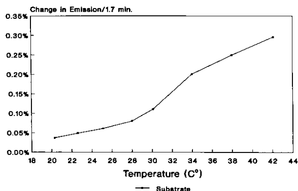
Fig. 8. Rates of autohydrolysis of the substrate CBZ-L-Arg-MCA, 0.20 mMol in TRIS-HCl buffer in relation to temperature in the assay solution. TRIS-HCl buffer 0.1 Mol, pH 8.0, \delta t = 1.7 min., excitation 380 nm, emission 440 nm
