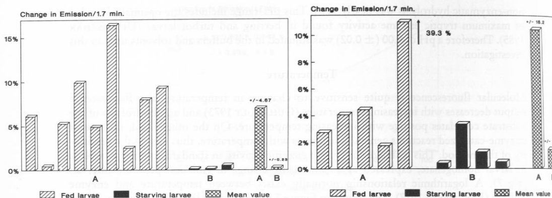
Fig. 9, left. Tryptic enzyme activity of 25-day-old fed and starved turbot larvae reared in the laboratory. Each bar gives the enzyme activity of an individually measured larva. The starving larvae were deprived of food for 7 days. Analytical procedure as described above
