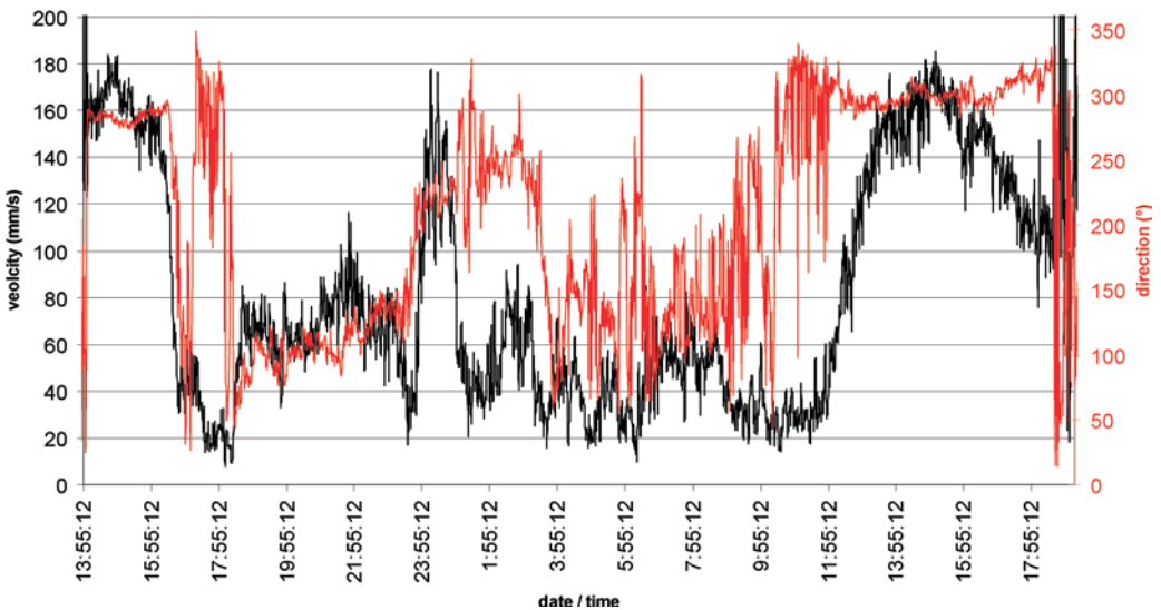
Fig. 7. 28-hour high resolution bottom water ADCP record from site 194. The left y-axis shows the current velocities in mm/second while the y-axis on the right shows current directions between 0^{\circ} and 360^{\circ} .
