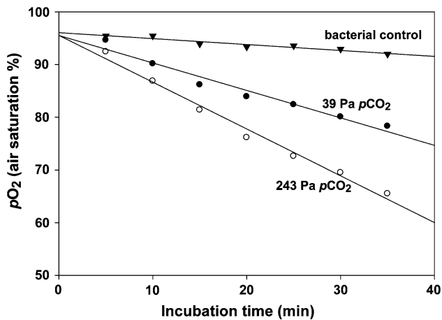
Fig. 1 Representative courses of pO_2 in the respiration chambers during measuring intervals between 5 and 35 min. Triangles represent the pO_2 change in a bacterial control. Black and white dots represent courses for mussels of the 39 and 243 Pa pCO_2 treatments, respectively
