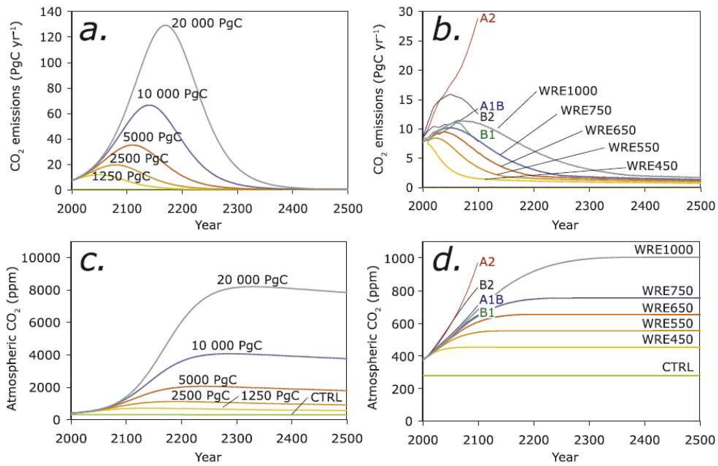
Fig. 4: (a) CO 2 emissions scenarios releasing from 1250 to 20,000 Pg C (4580–73,300 Pg CO 2 ) to the atmosphere after year 2000 (1Pg=1Gt). (b) CO 2 emissions specified for the Special Report on Emissions Scenarios (SRES) A1, A2, B1, and B2 pathways (IPCC 2000) and allowable emissions calculated with an ocean model from WRE (Wigley et al. 1995) CO 2 stabilization scenarios. (c) Model-predicted atmospheric CO 2 contents (ppm) for the emission pathways shown in (a). (d) Atmospheric CO 2 (ppm) predicted for the SRES emission pathways and specified for the WRE stabilization scenarios. From Caldeira and Wickett (2005).
