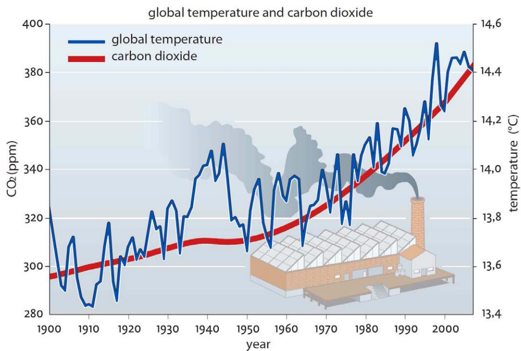
Fig. 1: Observed annual globally averaged SAT (°C, blue line) taken from HadCRU3 and smoothed atmospheric carbon dioxide concentration (ppm, red line) during 1900-2008.
