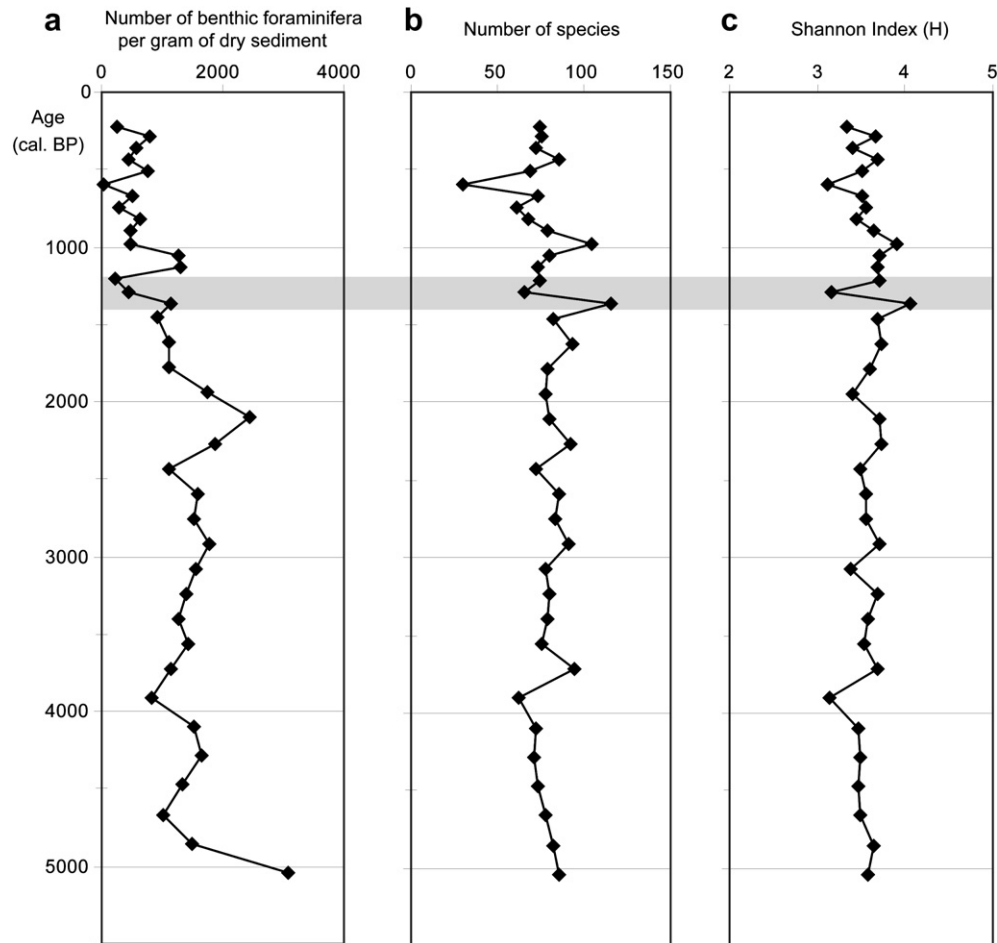
Fig. 4. Variation with age (cal. BP) in core 8 in: a) number of benthic foraminifera per gram of dry sediment; b) number of species; and c) Shannon index of diversity. The grey band denotes the transitional stage between the two identified depositional units.
