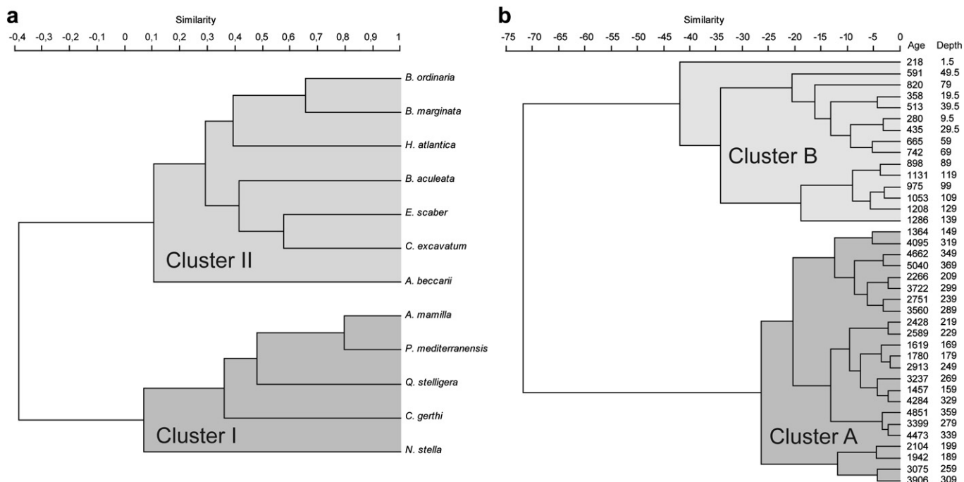
Fig. 7. Dendrogram classification resulting from cluster analyses based on the 12 species with relative abundances higher than 5% in at least one sample: a) Foraminiferal assemblages produced by R-mode analysis (correlation method joined by UPGMA); b) Sample associations produced by Q-mode analysis (Ward's method).
