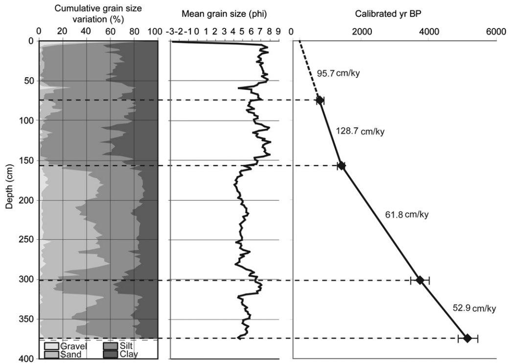
Fig. 2. Variation in cumulative grain size, mean grain size, age, and sedimentation rate with depth (cm) in core 8.
