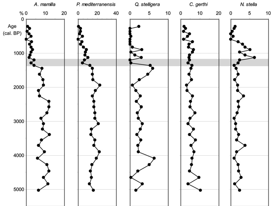
Fig. 5. Variation in the main species relative abundance (%) in the lower unit with age (cal. BP) in core 8. The grey band denotes the transitional stage between the two identified depositional units.
