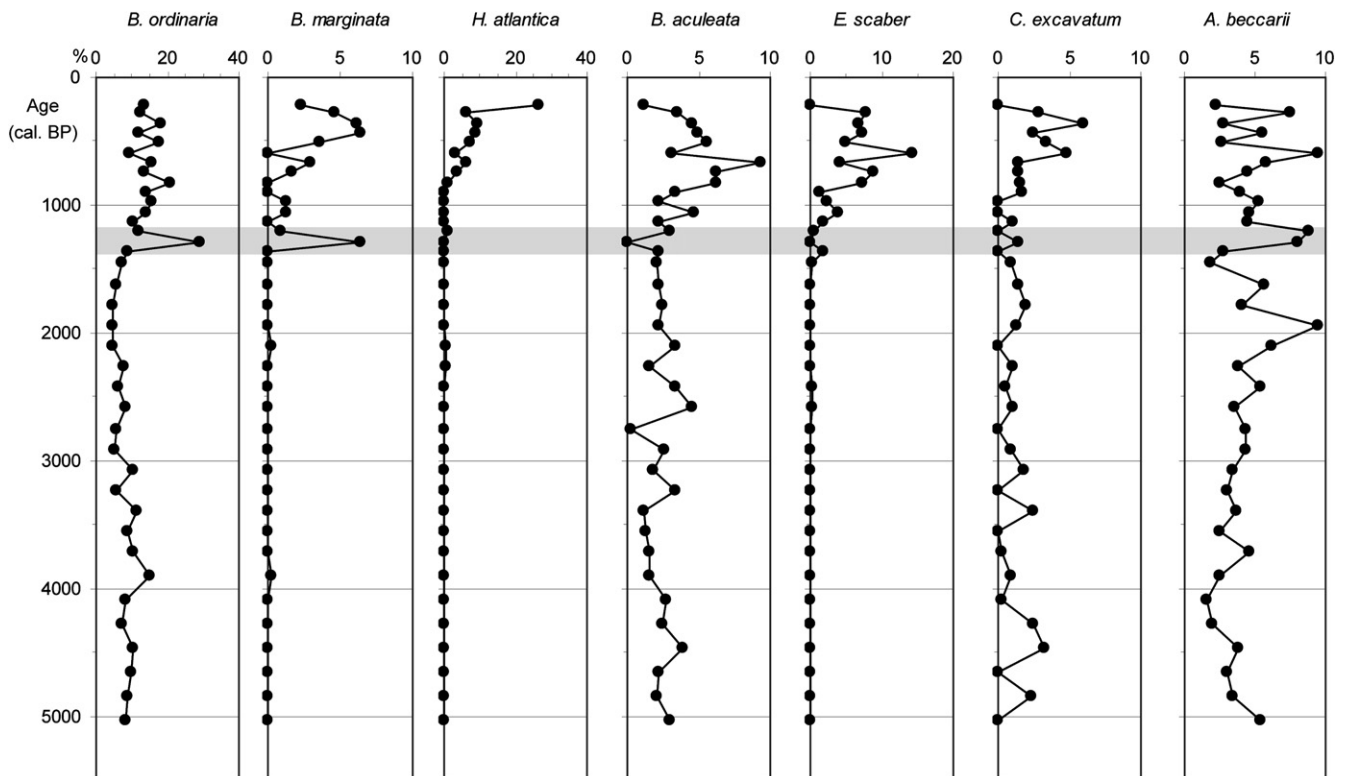
Fig. 6. Variation in the main species relative abundance (%) in the upper unit with age (cal. BP) in core 8. The grey band denotes the transitional stage between the two identified depositional units.
