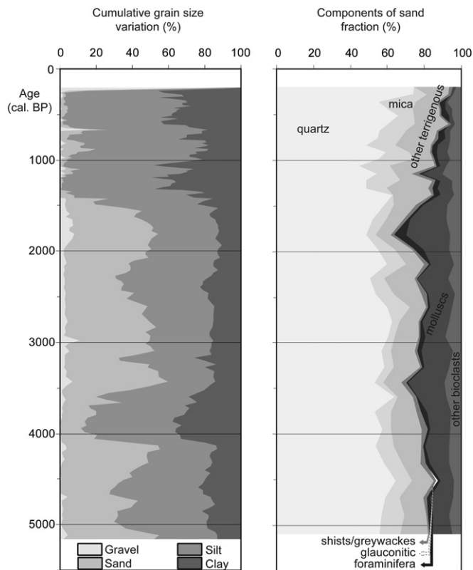
Fig. 3. Variation in cumulative grain size and components of the sand fraction with age (cal. BP) in core 8.
