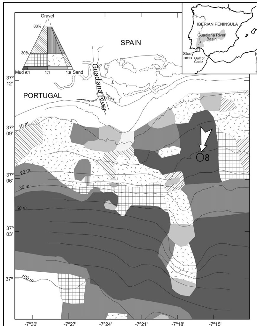
Fig. 1. Location of core 8 and the distribution of surface sediments on the continental shelf off the Guadiana River. Adapted from Gonzalez et al. (2004).
