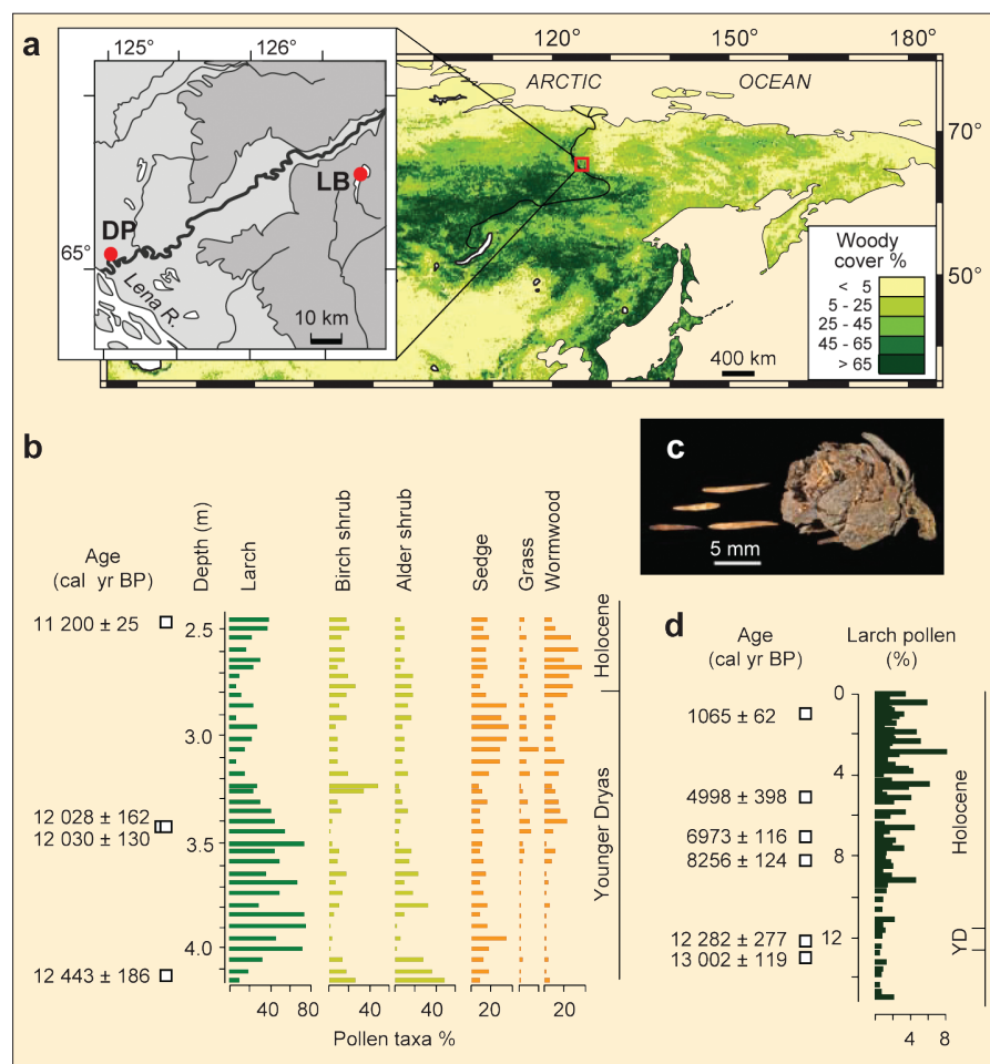
Figure 1: a ) Location of Dyanushka Peat (DP) and Lake Billyakh (LB) study sites (left) in the boreal forest belt of eastern Siberia (right, modified from Tarasov et al., 2007); b ) Pollen diagram of the lowest part of the DP section, showing percentages of selected tree, shrub and herbaceous taxa and the calibrated radiocarbon ages (68% range); c ) Photo of larch cone and needles from 340-345 cm depth in DP, dated to 12,030±130 (Poz-28087) and to 12,028±162 cal yr BP (KIA26015), respectively (after Werner et al., 2009); and d ) Chart showing the occurrence of larch pollen during ~15 ka in the short core from LB (after Müller et al., 2009). Radiocarbon years before present were converted to calendar years using the CalPal program (Danzeglocke et al., 2008).
