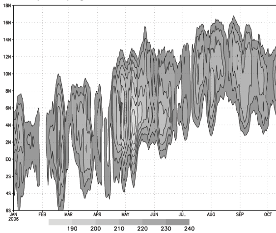
Figure 2: Time-latitude cross-section of the OLR field averaged on 10°W-10°E from 1st January to 11th October 2006. A moving average on +/-3 days have been applied to smooth the signal. The coastline is located approximately at 5°N.
