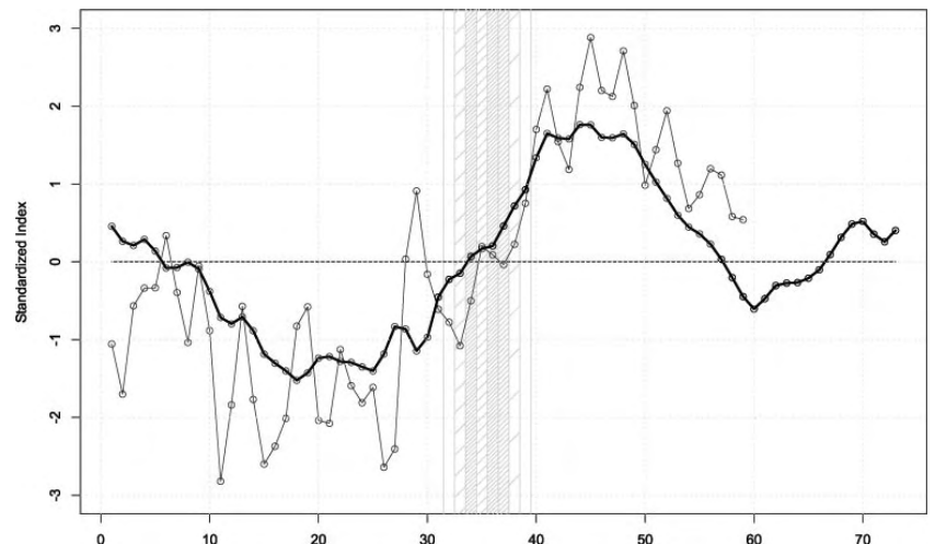
Figure 3: Time series of the 5-day monsoon index (see text for more details). The thick (thin) line represents the averaged index over the period 1979-2000 (the 2006 index). Vertical bars represent the probability function defined in Sultan and Janicot (2003). The x-axis labels are expressed in pentad.
