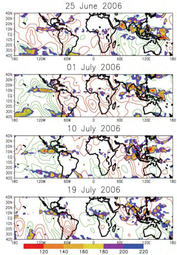
Figure 4: Daily OLR values (shaded) and 200 hPa NCEP velocity potential anomalies (relative the period 1979-1999) on 25th June, 1st July, 10th and 19th July 2006. Green (red) contours means upper-level large-scale divergence (convergence), by step of 2 \times 10^6 \text{ m}^2 \cdot \text{s}^{-2} (the zero isolines are not displayed).
