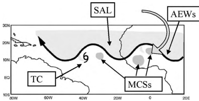
Figure 1: Key weather systems in the West African and Tropical Atlantic regions. Solid line represents a streamline at the level of the AEJ around 600hPa. Dark shading represents embedded MCSs and light shading indicates the location of the Saharan Air Layer (SAL). The large arrow represents the mean dry intrusions track seen in 2006.
