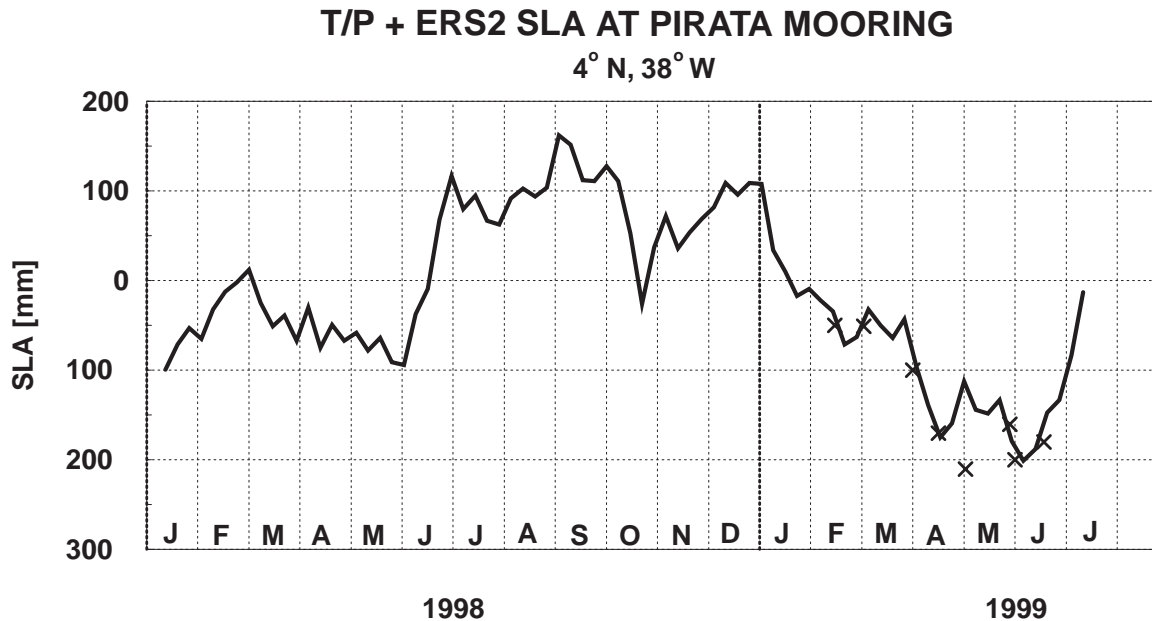
Fig. 3: Sea level anomalies observed by TOPEX/Poseidon and ERS-2 for 4°N, 38°W (solid line) and dynamic height anomalies from PIRATA temperatures, using a climatological T-S relationship (crosses). The difference between SLA and dynamic height is set to zero for February 1999.
