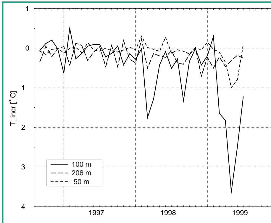
Fig. 4: Temperature increment obtained from the assimilation of subsurface temperatures in the area of 4°N, 38°W at 100 m depth (solid), 206 m depth (long-dashed), and at 50 m depth (dashed).
