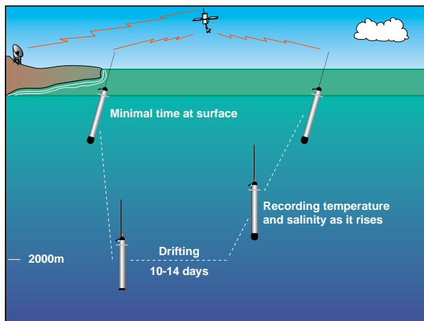
Figure 2: Schematic diagram of a ARGO float cycle
