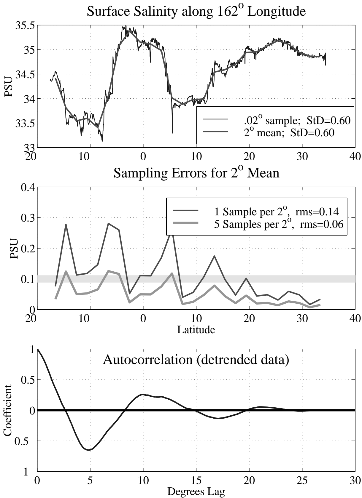
Fig. 3a: Top: meridional SSS section along 162°E; middle: sample errors; bottom: auto-correlation function.
