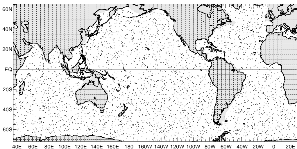
Figure 1: An example of the projected global distribution of ARGO floats
