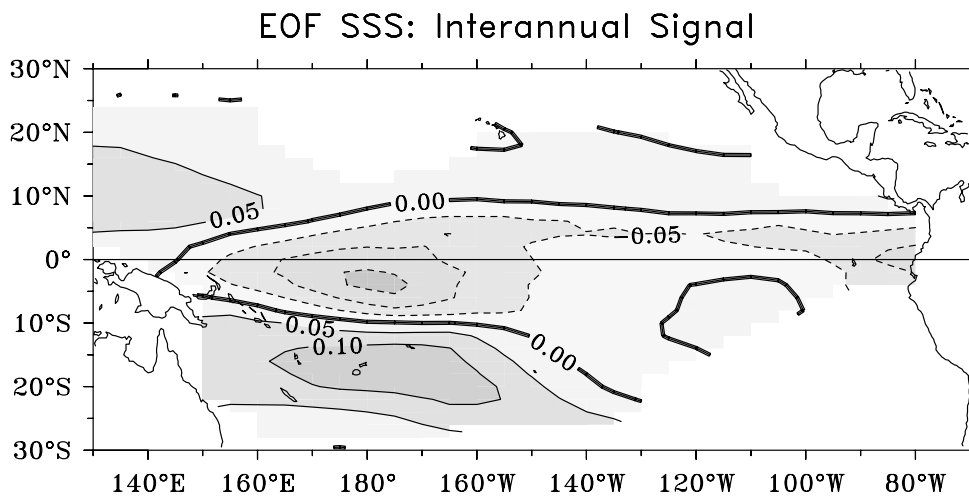
Figure 2: Spatial pattern of the interannual EOF in SSS. The time function (not shown) is in phase with the SOI. (Adapted from Delcroix, 1998).
