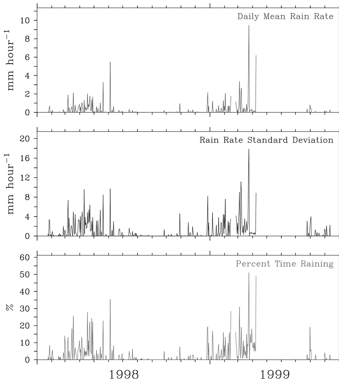
Figure 2b: Rainfall parameters for the PIRATA buoy at 0°, 35°W
