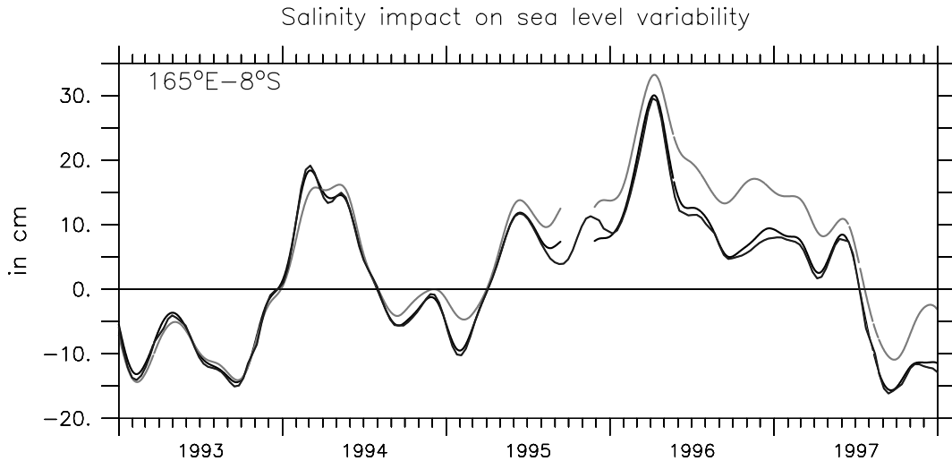
Figure 1: Time series of dynamic height with (dark curve) and without (upper light curve) salinity variability, compared with TOPEX/Poseidon (lower light curve) (from Maes and Behringer, 1999).
