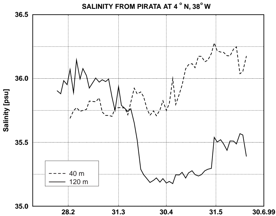
Figure 2: Time series of salinity as observed from the PIRATA mooring at 4°N, 38°W at 40 m depth (dashed) and at 120 m depth (solid).
