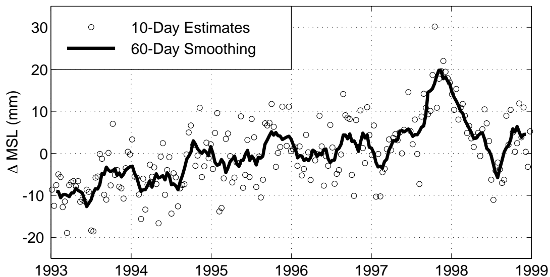
Figure 1: Time series of the global mean sea level computed from T/P (after Nerem and Mitchum, 1999). A mean sea level estimate is computed for each 10-day T/P cycle, and these points are shown by open circles. The solid curve is a 60-day running mean of the 10-day points that emphasises the low frequency variability in the curve.
