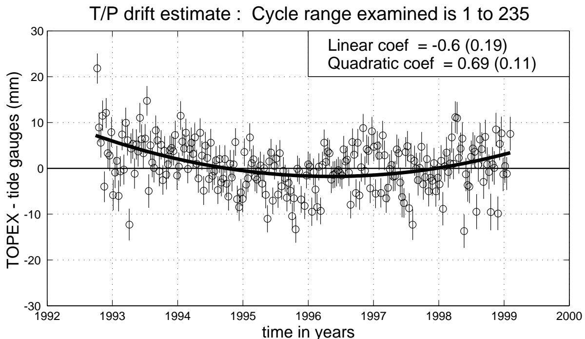
Figure 4: The present estimate of the estimate of the T/P drift error based on the global tide gauge network. All of the tide gauges shown as open circles in Figure 3 were used in this analysis, although some did not prove useful. Additional details on the method used to derive this estimate are given by Mitchum (1998) and in Nerem and Mitchum (1999). The solid curve is from a weighted least squares fit of a quadratic curve to the 10-day estimates given by the open circles.
