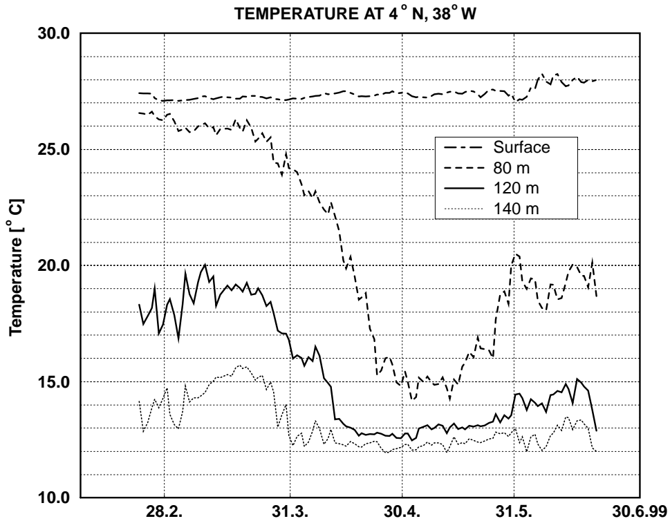
Figure 1: Time series of temperature as observed from the PIRATA mooring at 4°N, 38°W for the surface (dash-dotted), at 80 m depth (dashed), at 120 m depth (solid), and at 140 m depth (dotted).
