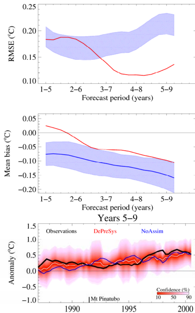
Figure 3: Predictions of five year averages of surface temperature over western Europe, from a set of 80 ensemble hindcasts from the DePreSys_Orig system. Each prediction is based on 16 simulations obtained by pooling the four member ensemble from the relevant start date with those started one, two and three seasons earlier. The top panel shows the root-mean squared error of the ensemble mean DePreSys_Orig hindcasts (red curve), compared against the 5-95% confidence range of values diagnosed from the parallel set of DePreSys_NoAssim hindcasts which use the same projections of external forcing agents as DePreSys_Orig, but are started from initial states independent of observations. The middle panel shows corresponding results for the mean bias in the predictions, and the bottom panel shows time series of the ensemble mean (white curve) and 5-95% confidence range (red shading) of DePreSys_Orig predictions for 5-9 years ahead, alongside verifying observations (black curve) and the ensemble mean predictions of DePreSys_NoAssim (blue curve).
