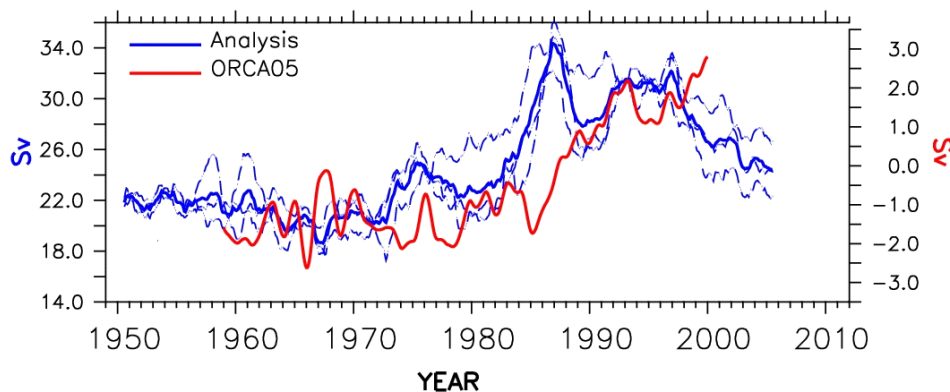
Figure 2: Analysed fields of the North Atlantic maximum meridional overturning stream function at 40°N. Dashed blue lines indicate the individual ensemble members and the thick solid blue line the ensemble mean. The red line is from a forced ocean only simulation with the NEMO model (ORCA05 resolution).
