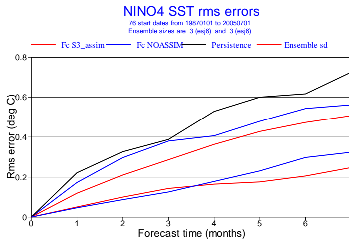
Figure 1: Positive impact of the data assimilation in terms of skill of seasonal forecasts of SSTs in the Niño4 region of the western tropical Pacific in ECMWF's system 3. Root-mean squared error of forecasts initialised with the new S3 ocean re-analysis (red solid line), of forecasts initialised with an ocean analysis without assimilating observations (blue solid line), of a persistence reference forecast (black dashed line) and the ensemble spread (red and blue dashed lines) versus forecast lead time. Figure from Balmaseda et al. , 2007c.
