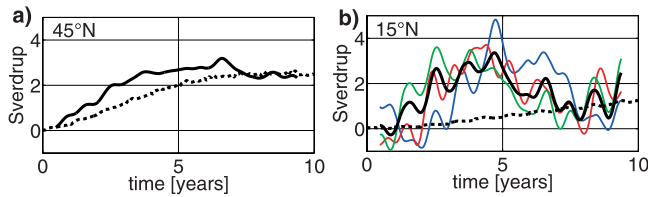
Figure 1. MOC anomaly ( Sv ) of RESP 4/3 (black dashed line) and RESP 1/3 (black solid line) - a mean of three ensemble members - at (a) 45^\circ N and (b) 15^\circ N . The thin coloured lines denote the response of each ensemble member. MOC is defined as the zonally integrated, southward-transport of deep water below 1500 m. All time series in all figures are 2-year low-pass filtered to remove the seasonal cycle.
