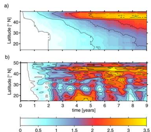
Figure 2. MOC anomaly ( Sv ) in the NAO response experiments (a) RESP 4/3 and (b) RESP 1/3. The latter representing the mean of three ensemble members.
