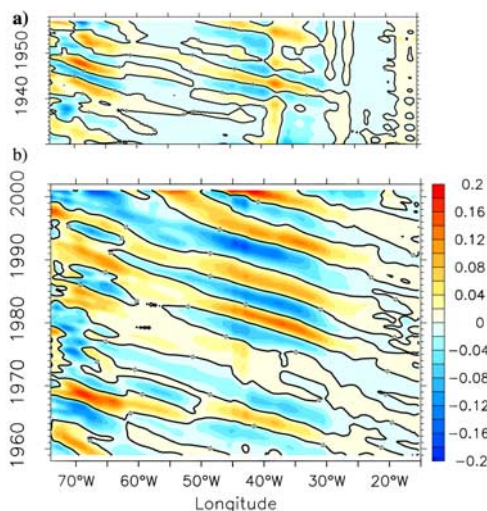
Figure 4. Meridional velocity anomalies (cm/s) in 2500 m depth along 27°N, for (a) CLIM and (b) HEAT.
