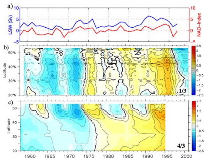
Figure 3. (a) Comparison between the rate of the Labrador Sea convection as given by the renewal of LSW (in Sv, blue) and the NAO-Index (red). Below: MOC anomaly (Sv) of the model experiments forced by the NCEP-based heat flux for (b) HEAT 1/3 and (c) HEAT 4/3.
