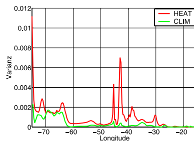
Figure 5. Variance of meridional velocity anomalies ( \text{cm}^2/\text{s}^2 ) in 2500 m depth along 27°N, for CLIM and HEAT.
