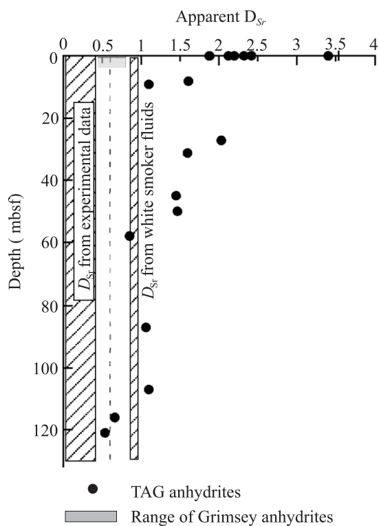
Fig. 8. Apparent D_{Sr} of Grimsey anhydrites compared to downcore variation of D_{Sr} in TAG samples and D_{Sr} from white smoker fluid and experimental data (from Shikazono and Holland, 1983; Mills and Tivey, 1999). Low D_{Sr} at TAG represents precipitation from a fluid which was not evolved; high D_{Sr} corresponds to an evolved fluid (i.e., continued mixing of a rising black smoker fluid with deeply entrained and heated seawater and subsequent anhydrite precipitation). Grimsey anhydrites have low D_{Sr} and are probably similar to D_{Sr} from a white smoker fluid at TAG.
