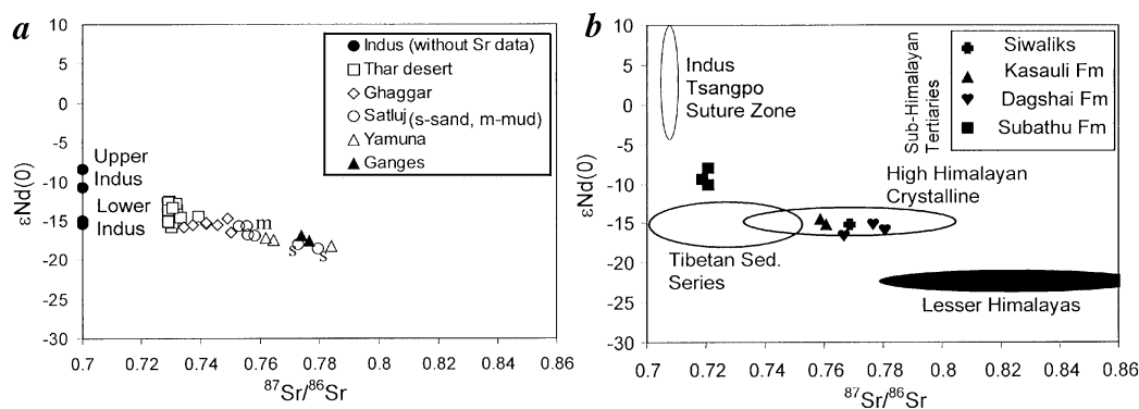
Figure 2. a , Nd–Sr isotopic composition of the sediments of northwestern India. Geochemically, the Ghaggar and Thar sediments are distinct for their lesser radiogenic Sr and more radiogenic Nd isotopes. These sediments show more affinity to the marine Subathu Formation containing juvenile ITSZ components, present in the Ghaggar catchment. The present isotopic composition of the Thar is explained by mixing of the HHC-dominated Dagshai, Kasauli and Siwalik sediments with the Subathu sediments, all present at the Ghaggar catchment. An analogous case is the Nd of lower Indus sediment, which is explained by mixing of ITSZ-dominated upper Indus with the HHC-dominated Satluj sediments. b , Nd–Sr isotopic distribution for different tectonic units of Himalayas (15, 16). \epsilon_{Nd}(0) calculated at time t = 0 for CHUR ^{143}Nd/^{144}Nd = 0.512638 .
