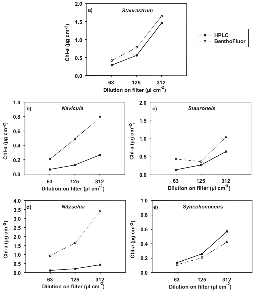
Fig. 4. Total chlorophyll- a concentrations ( \mu\text{g cm}^{-2} ) of different microalgae culture suspensions measured with HPLC and the Benthofluor. Microalgal cultures measured: a) Staurastrum sp. (green group), b, c, d) Navicula sp., Stauroneis sp., Nitzschia sp., (brown group) and e) Synechococcus sp. (blue group).
