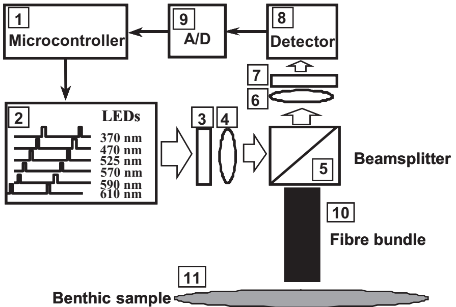
Fig. 2. The Benthofluor components: (1) microcontroller, (2) six light-emitting diodes, (3) short-pass filter to block red and IR emission, (4) focussing lens ( f = 25 mm), (5) beamsplitter, (6) focussing lens, (7) band-pass filter, (8) integrated photomultiplier, (9) 12-bit AD-converter (conversion rate of 100 kHz), (10) fibre bundle and (11) benthic sample.
