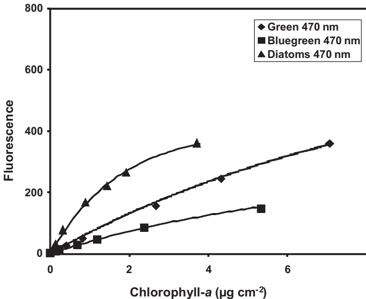
Fig. 3. Fluorescence intensities of three spectral algal groups at various concentrations at an excitation wavelength of 470 nm.
