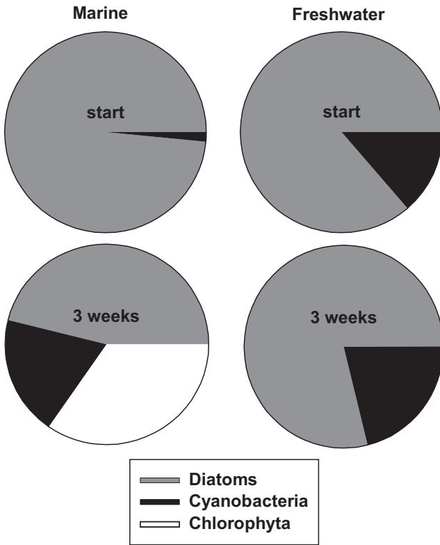
Fig. 6. Major taxonomic components of the microphytobenthos in the marine (left) and the freshwater (right) incubations given as proportions (%) from the total algal at the beginning (top) and after 21 days (bottom) of incubation.
