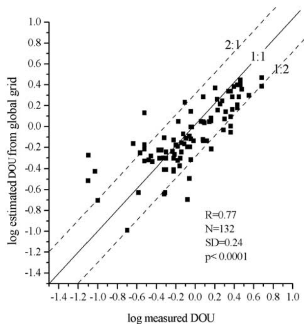
Figure 8. Comparison of oxygen flux measurements and estimated flux values (DOU) after applying regression fits to the regular TOC grid. Estimated values were queried from the global grid (DOU) before calculating the J_{\text{POC}} = 0.77 \times \text{DOU} (see Figure 7).
