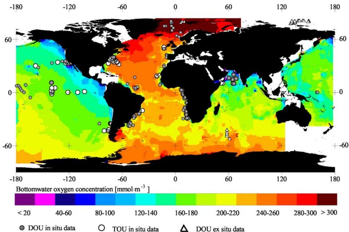
Figure 2. Distribution pattern of the bottom water oxygen concentration measured in \text{mmol m}^{-3} and based on \sim 6700 bottle data (WOCE, GEOSECS). Gray circles: in situ DOU data ; white circles: in situ TOU data ; triangles: ex situ DOU data. Only data used in the regression analyses ( w_d > 1000 m) are displayed.
