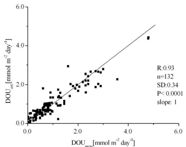
Figure 6. Estimation accuracy of all regression fits within 83.5^{\circ}\text{N} – 85^{\circ}\text{S} , displayed as estimated DOU ( \text{DOU}_{\text{est}} ) versus measured DOU ( \text{DOU}_{\text{meas}} ). Bisecting line shows regression fit.
