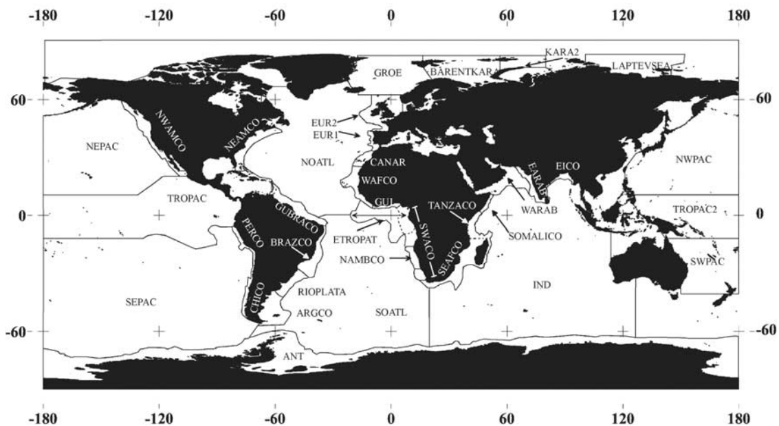
Figure 1b. Updated discretization of the global ocean in 33 benthic TOC-based provinces (TROPAC/TROPAC2; NEPAC/NWPAC; SEAPAC/SWPAC; each pair is combined to one province) [Seiter et al., 2004].
