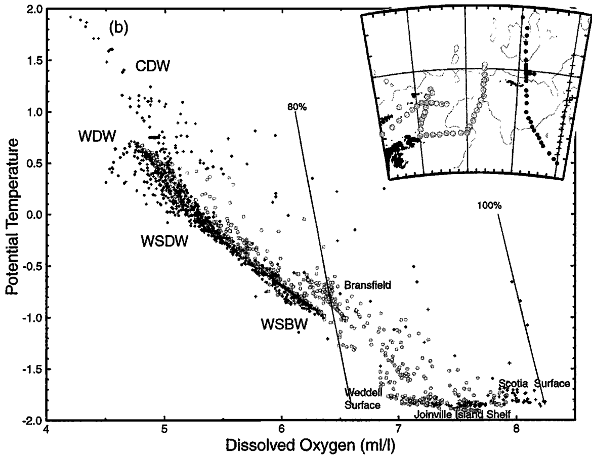
Figure 4. Potential temperature ( ^{\circ}\text{C} ) versus (a) salinity (CTD data) and (b) oxygen ( \text{mL/L} ) (oxygen bottle data) for all Nathaniel B. Palmer cruise 97-5 CTD/rosette stations (shaded circles). Data from the 44^{\circ}\text{W} section are highlighted as solid symbols.
