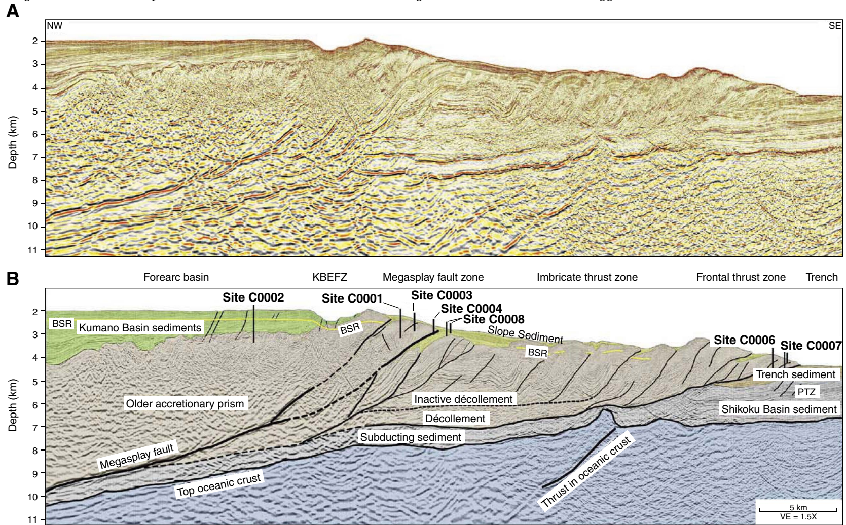
Figure F3. Composite seismic line extracted from 3-D seismic volume, reproduced from Moore et al. The line crosses through (or near) all Stage 1 drill sites (Fig. F1). A. Uninterpreted depth section processed with prestack depth migration. B. Interpreted version of A. Only a few representative faults are shown. Dashed lines = less certain fault locations. Morpho-tectonic zones are shown between the two sections. KBEFZ = Kumano Basin edge fault zone, PTZ = protothrust zone, BSR = bottom-simulating reflection, VE = vertical exaggeration.
