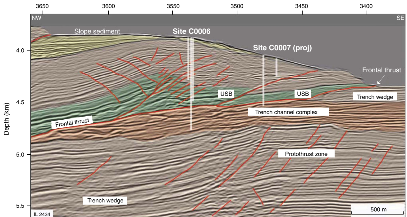
Figure F4. Inline seismic section for the frontal thrust region, Sites C0006 and C0007 (reproduced from Moore et al.). USB = upper Shikoku Basin facies sediment package.
