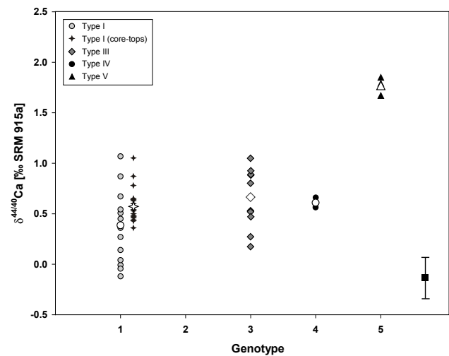
Fig. 2. Genotypes of N. pachyderma (sin.) plotted vs. Ca isotope composition showing that genotype has a no considerable effect on \delta^{44/40}\text{Ca} . The mean \delta^{44/40}\text{Ca} values for each genotype are presented as open symbols. Note that within uncertainties, the mean \delta^{44/40}\text{Ca} values for genotype I, III and IV are indistinguishable from each other. The uncertainty on the \delta^{44/40}\text{Ca} values is given in the right corner.
