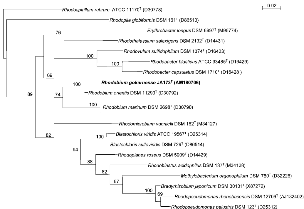
Fig. 1. Dendrogram depicting the phylogenetic relationships of strain JA173 T within the family Rhodobiaceae determined using 16S rRNA gene sequence analysis. Bar, 2 substitutions per 100 nucleotides.
