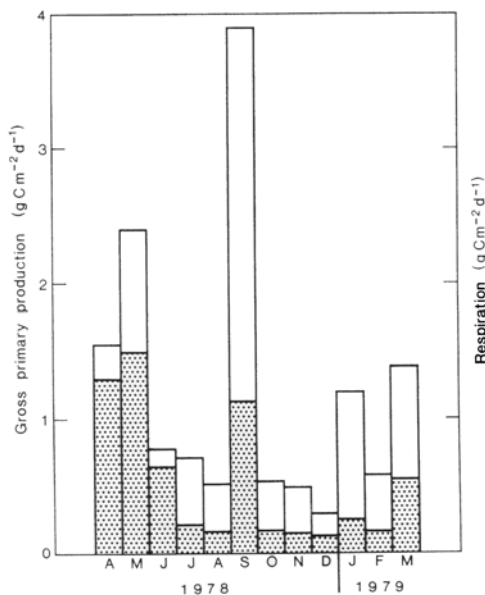
Fig. 2. Integrated gross primary production (PPg), net primary production (PPn) and respiration (R) of the photic layer (down to 1 m). PPg is represented by the total length, PP n by the upper part and R by the dotted part of columns.
