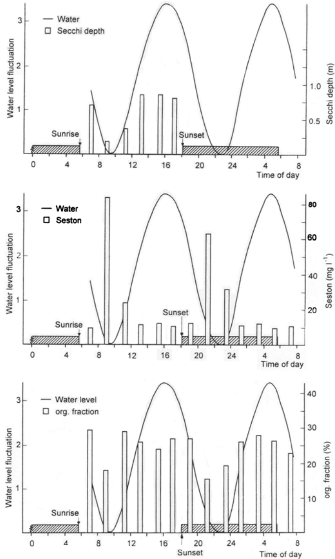
Fig. 4. Tidal variations of water level, Secchi depth (a), total seston concentration (b) and fraction of organic seston (c) on 25 June.
