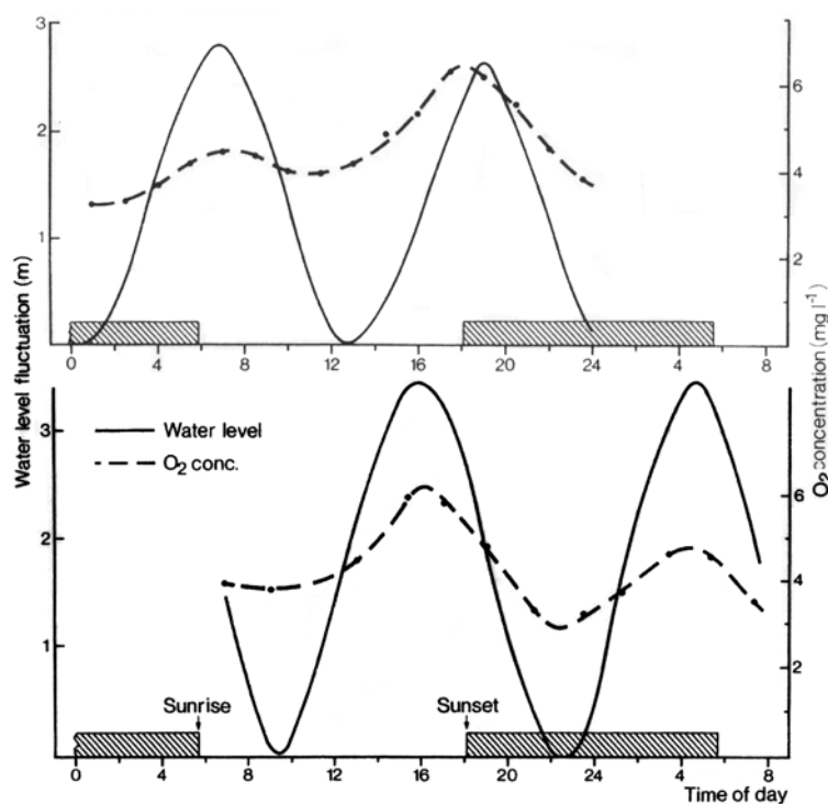
Fig. 3. Tidal variations of water level and oxygen concentration in the mouth of the main channel of a mangrove forest on 31 May (upper part) and 25 June (lower part).
