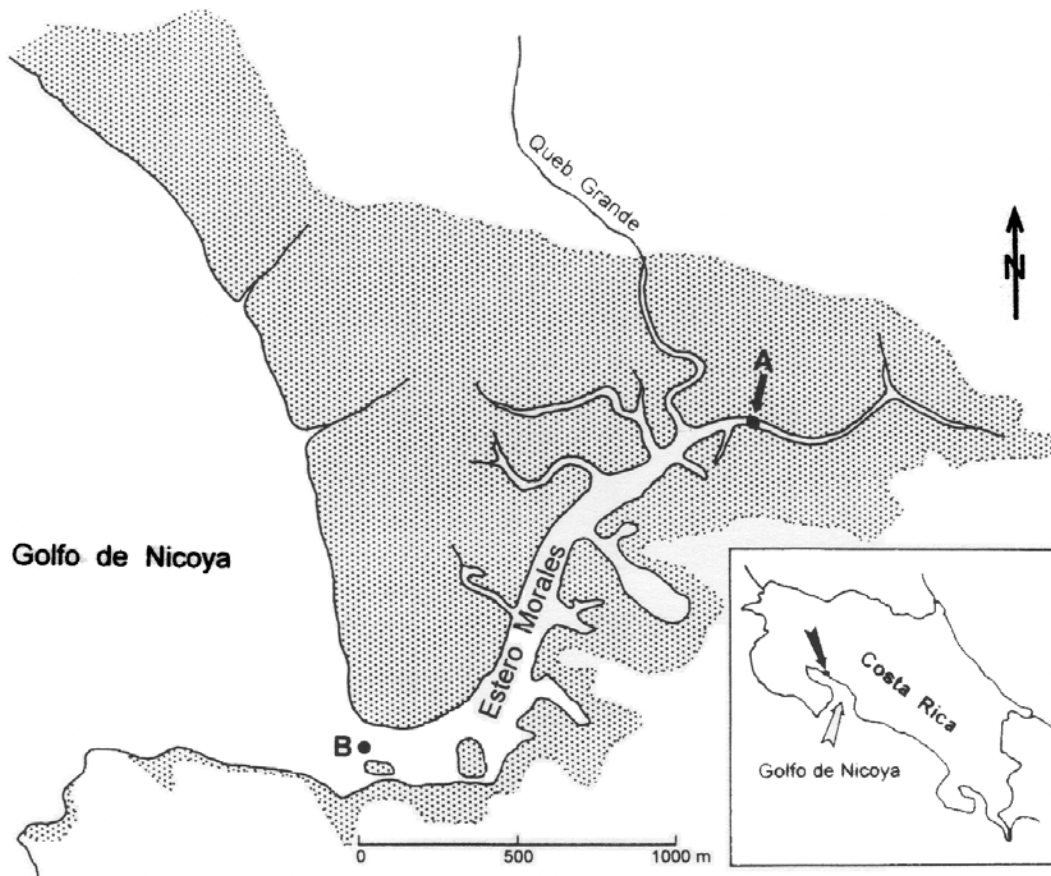
Fig. 1. Location of the study site. At station A the seasonal study was performed, station B was the location of the additional measurements.
