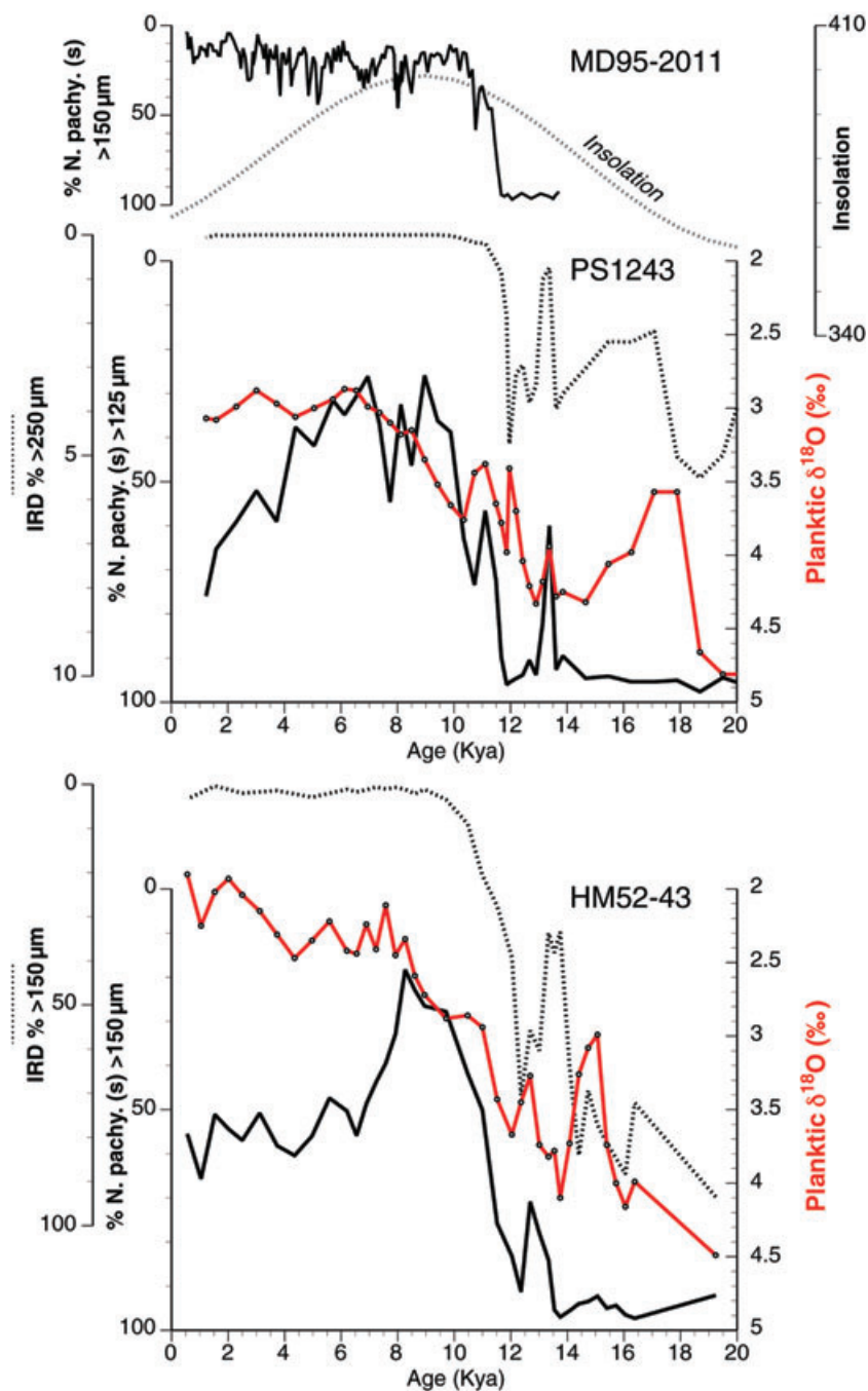
Fig. 2. Proxy record from the Norwegian Sea showing the evolution of surface water masses, as indicated by the proportion of the polar planktic foraminifer Neogloboquadrina pachyderma (s), its oxygen isotope composition and the relative quantity of iceberg-rafted debris (IRD). The records are shown alongside the northern summer insolation 65^{\circ}\text{N} ( \text{W m}^{-2} ; Berger 1978), when Arctic-sub-Arctic regions usually show the least seasonal sea-ice cover (from mid-July through to August).
