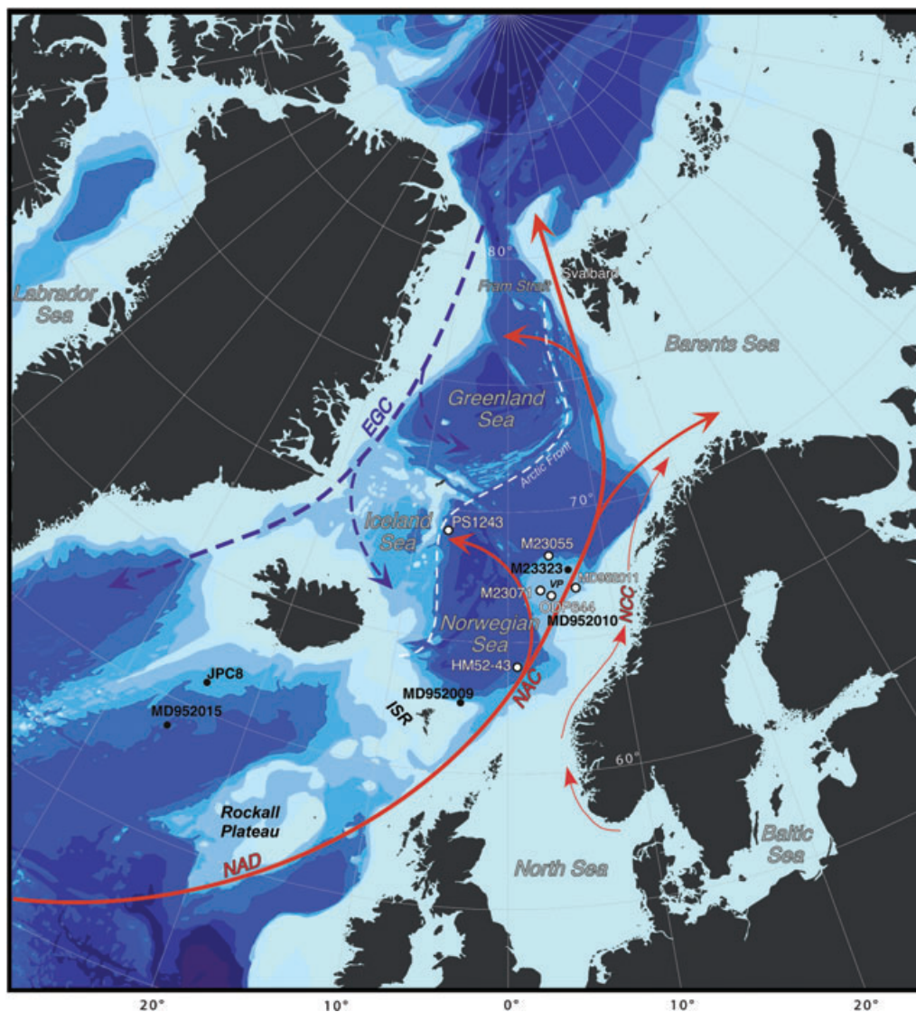
Fig. 1. Map of the subpolar and polar North Atlantic region showing a schematic overview of the meridional surface ocean circulation. The positions of sediment cores studied (large white labels) and discussed in this work (black labels) are indicated. MD95-2010 and ODP644 share the same position. Abbreviations: EGC, East Greenland Current; ISR, Iceland–Scotland Ridge; NAC, Norwegian Atlantic Current; NAD, North Atlantic Drift; NCC, Norwegian Coastal Current; VP, Vøring Plateau.
