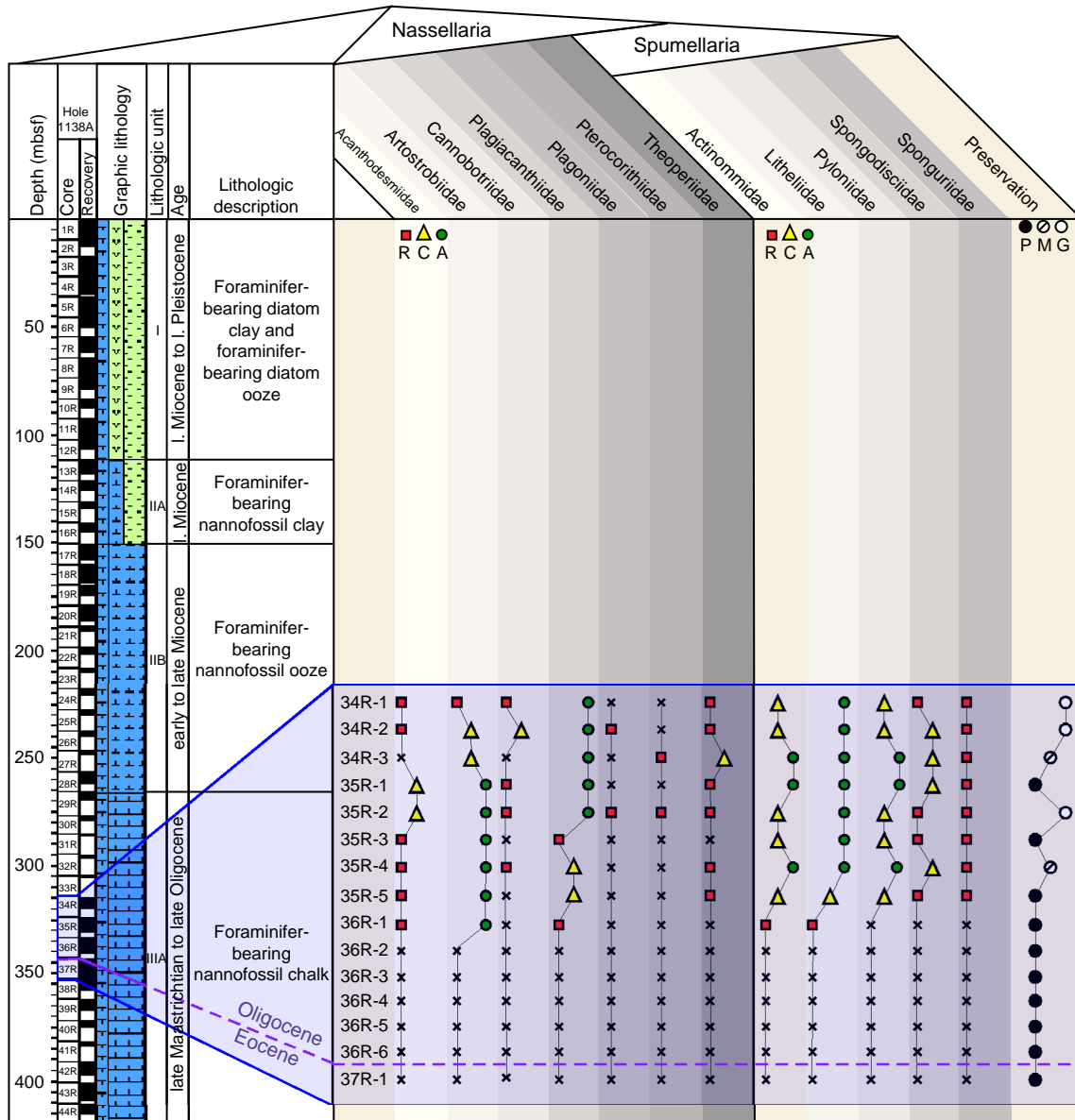
Figure F3. Family level faunal characteristics of studied samples (late Eocene to Oligocene age) at Site 1138. Samples of early Eocene to Maastrichtian age were also studied but contained no radiolarians. Preservation: P = poor, M = moderate, G = good. Abundance: R = rare, C = common, A = abundant.
