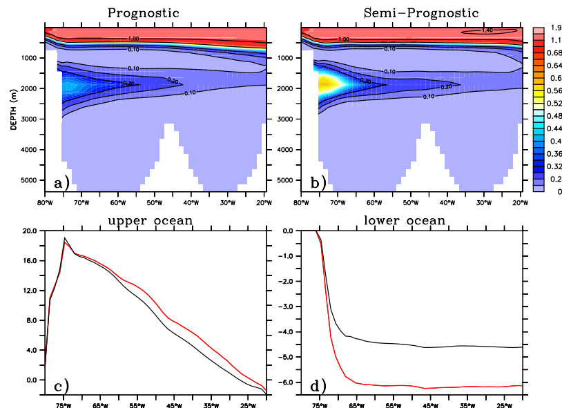
Figure 3. The concentration of CFC-12 along 24^{\circ}\text{N} in the (a) prognostic and (b) semi-prognostic model runs, corresponding to February 1997, in units of pmol/kg. (c) and (d) show the cumulative advective transport (positive northward) through 24^{\circ}\text{N} integrated eastwards from the western boundary for the upper (above 1000 m) and lower (below 1000 m) ocean in the prognostic (black) and semi-prognostic (red) model runs in units of 10^{-3} mol/s.
