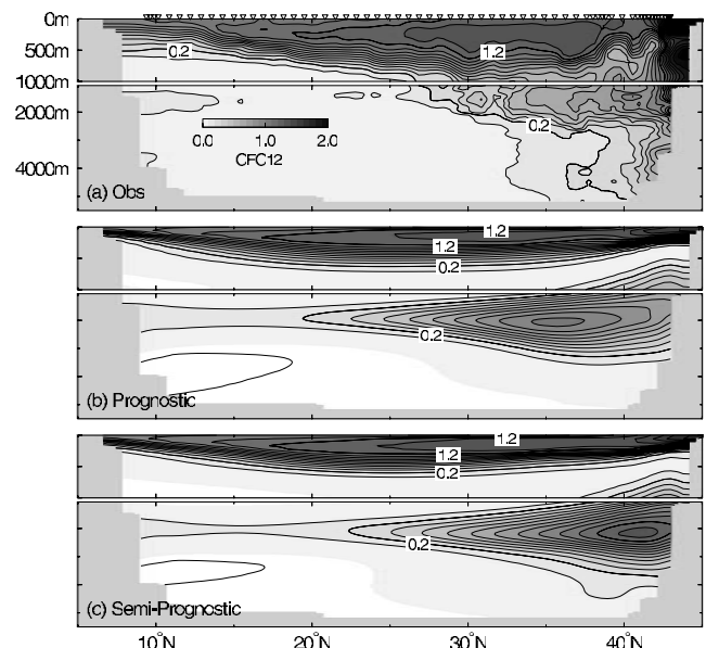
Figure 2. (a) The observed CFC-12 concentration in pmol kg -1 along a meridional transect A20 at 52°W in the North Atlantic in July/August of 1997 redrawn from the data set described by [Smethie et al. , 2000]. The time-mean CFC-12 concentrations in pmol kg -1 averaged from the model results over July and August of 1997 along the same transect for (b) the prognostic model and (c) the modified semi-prognostic model.
