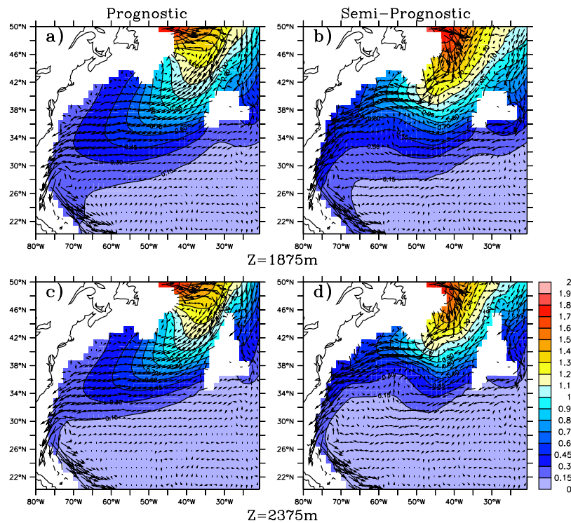
Figure 1. Monthly mean CFC-12 concentration in pmol/kg (color image) and horizontal velocity (arrows) over the western subtropical Atlantic in February of year 1990 at 1875 m depth in (a) the prognostic model and (b) the modified semi-prognostic model. (c) and (d) are as for (a) and (b) but at 2375 m depth.
