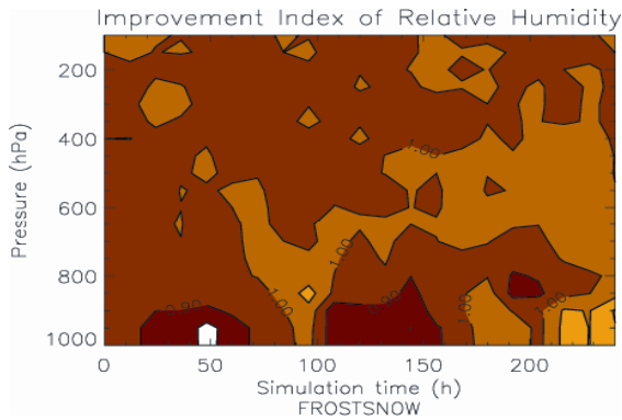
Figure 3: Improvement index, I , for predicted relative humidity; I > 1 degradation, I = 1 no change, I < 1 improvement.
