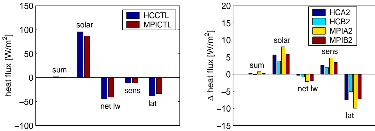
Figure 1 Left: Overall mean heat flux from the atmosphere to the ice/ocean system in components: Shortwave ('solar'), net longwave ('net lw'), sensible ('sens'), latent ('lat') and the sum of all components. Right: Differences between heat fluxes of scenario and control experiments. Figure taken from Döscher and Meier (2004).
