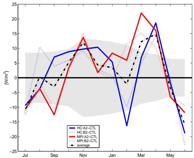
Figure 2: Difference between scenario and control run, positive into the ocean (the shaded area gives the approximate 95% confidence limit based on the standard deviations of the means). Figure taken from Döscher and Meier (2004).
