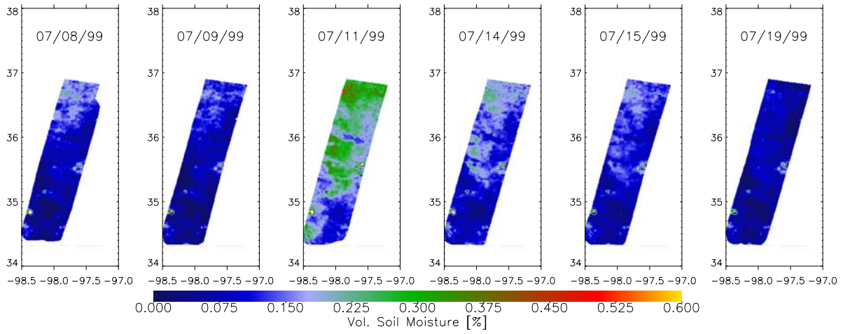
Fig. 1 (Drusch et al.): C-band derived soil moisture for the SGP99 experiment region (from Drusch et al. 2003)
