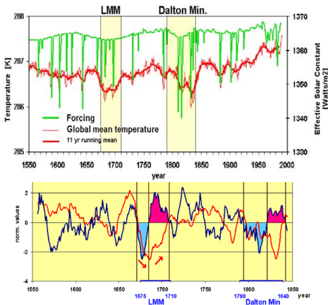
Fig. 1: Above: Model forcing (green) and global mean temperature (red). Below: NAO index (black) and global mean temperature after Fischer-Bruns et al. (2002).
