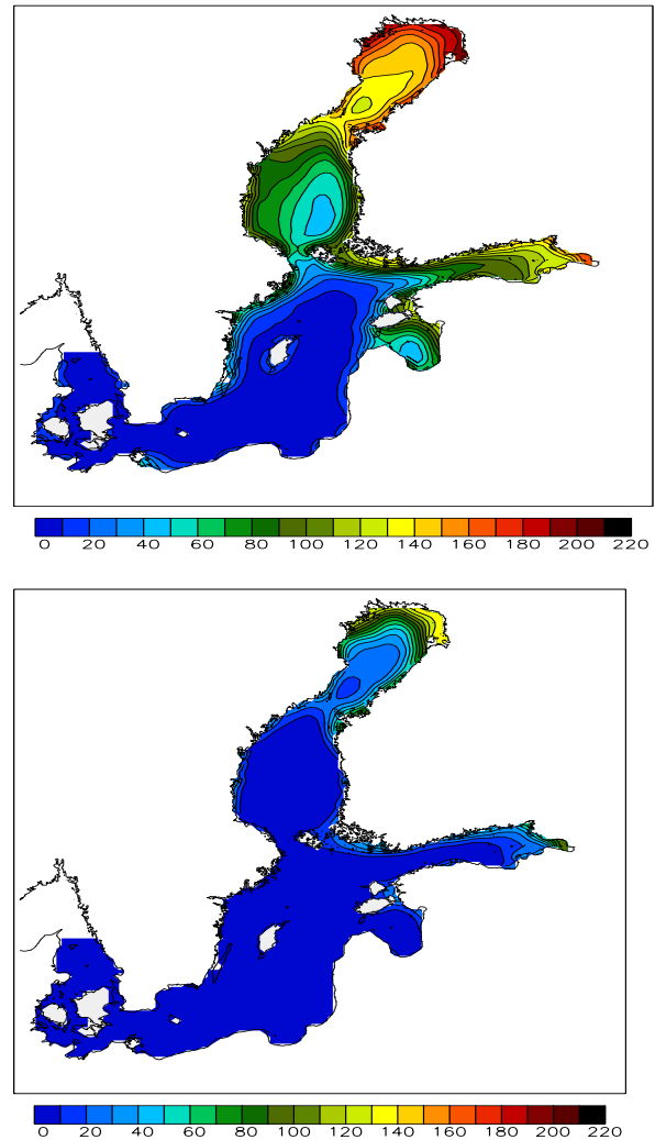
Figure 3: Mean number of ice days as average of HC and MPI. Top: Control run. Below: A2 scenario run. Figure taken from Meier et al (2004).
