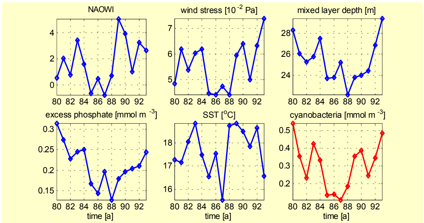
Fig. 3: Time series of the NAO winter index, the wind stress, the mixed layer depth, the excess phosphate, the SST and the biomass of cyanobacteria simulated with the present climate run (after Janssen et al. 2003). Mean of model area for all variables except NAOWI.
