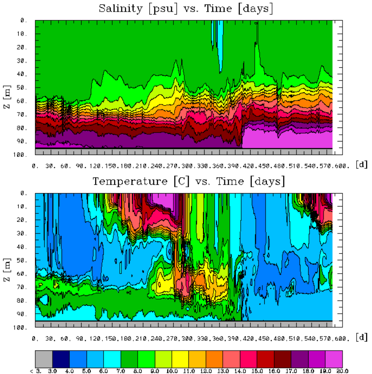
Figure 3 (BALTIMOS): Time series of vertical profiles of salinity [psu] (upper panel) and temperature [°C] at Bornholm Deep vs. time from January 2002 until July 2003 .
