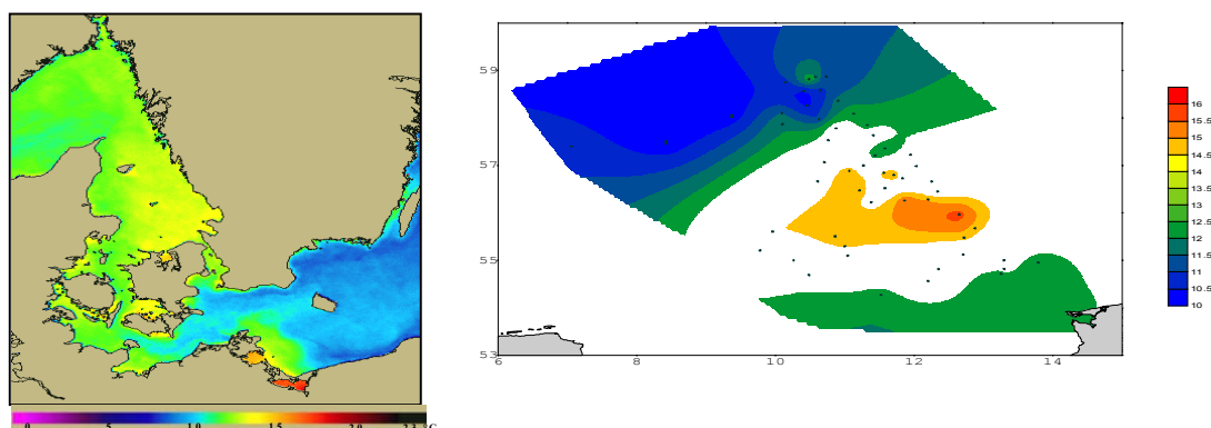
Fig. 2: Left: SST in May 2000 in the Skagerrak - Kattegat area from NOAA AVHRR (Data source: BSH, image processing, Siegel IOW). Right: SST calculated from alkenones in surface sediments (Blanz, in preparation).
