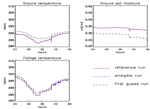
Figure 4: Data assimilation of soil and surface temperatures.
