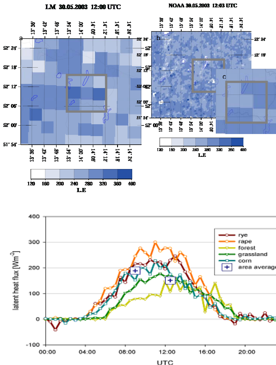
Fig. 4 (EVA-GRIPS): Evaporation over the LITFASS area on May 30, 2003, around noon, left: LM simula- tion, right: derived from NOAA data – (figure by C. Heret and F. Berger, TU Dresden)
