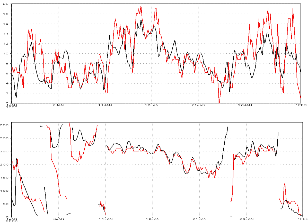
Figure 2: Wind speed [m/s] (upper panel) and wind direction [deg] (lower panel) for January 2003: Measurements at the SYNOP-Station "Arkona" (red) and BALTIMOS simulation for the appropriate grid box (black).
