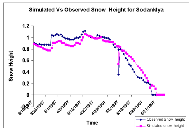
Figure 2: Snow height as simulated for and observed at Sodankylä, Finland 3/12-5/30/1997.
