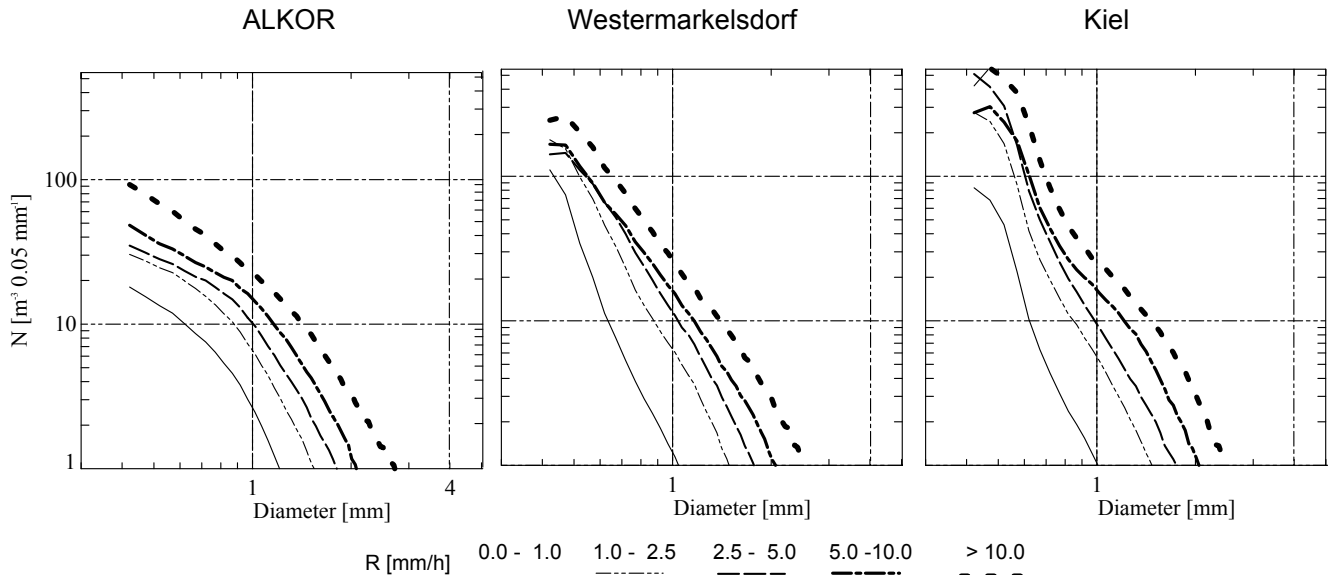
Figure 3 (APOLAS): Drop size distributions (1 min averages) measured at different sites representing maritime (ALKOR), intermediate (Westermarkelsdorf), and land (Kiel) conditions. The total number of rain events (minutes with rain detected) ranges from about 6000 to 25000 at the different sites.
