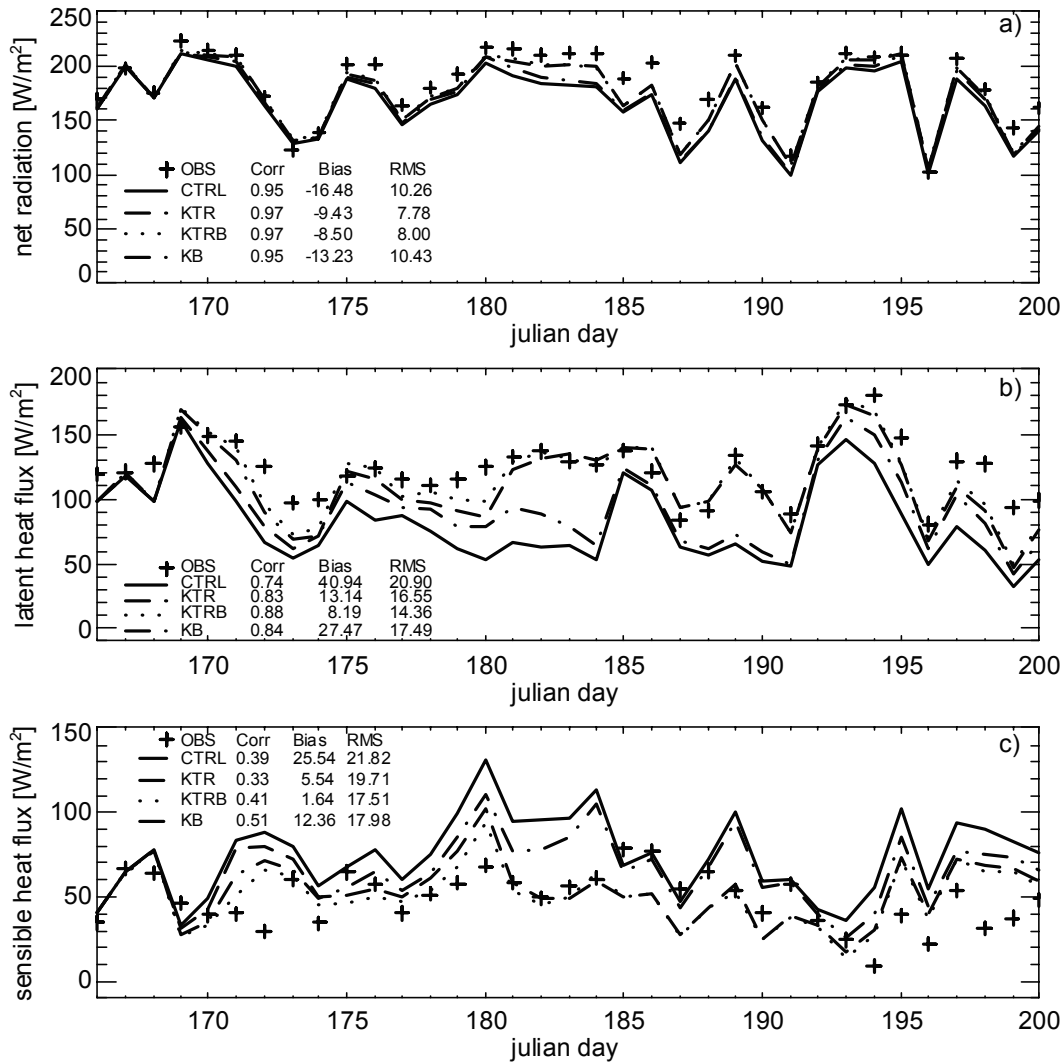
Fig. 2 (Drusch et al.): Temporal evolution for 15.6.-19.7.1997 of daily mean a) net radiation, b) latent heat flux, and c) sensible heat flux simulated by the control run (ctrl), assimilation runs with T_{2m} and rH (KTR), T_{brightness} (KB), and T_{2m} , rH and T_{brightness} (KTRB) (from Seuffert et al. 2003a).
