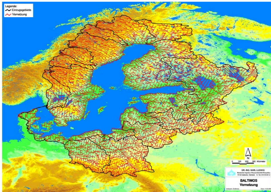
Figure 1: BALTEX catchment area and river routing scheme of BALTIMOS.
