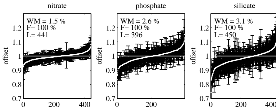
Figure 3. Offsets calculated for the crossovers in the CARINA-ATL data after adjustments have been applied. WM: the weighted mean of the offsets (see text); F: the percentage of offsets indistinguishable from 1 within their uncertainty; L: the number of crossovers.
