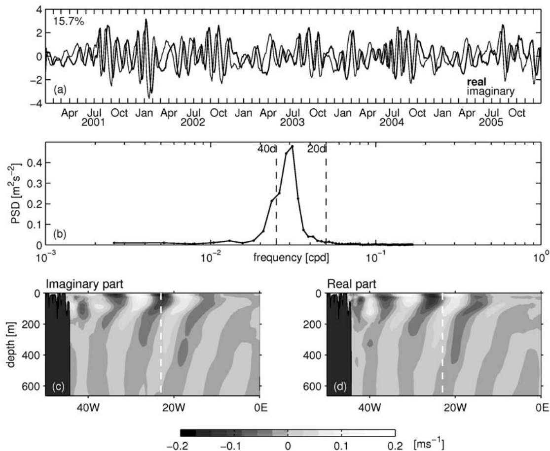
Figure 5. Principal oscillating pattern (POP) analysis using DAILY simulated meridional velocity along the equator. (a) Real (bold line) and imaginary part of the nondimensional coefficients of the first POP and (b) corresponding power spectral density. (c) Imaginary and (d) real part of the dominant POP pattern. The 23^{\circ}\text{W} longitude is marked with a dashed white line.
