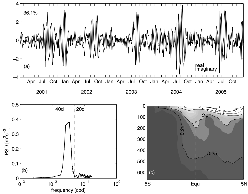
Figure 6. POP analysis using DAILY simulated meridional velocity along the 23°W section. (a) Real (bold) and imaginary part of the nondimensional coefficients of the first POP and (b) corresponding power spectral density. (c) Amplitude of the dominant POP, contours are in \text{cm s}^{-1} . The equator is marked with a dashed white line.
