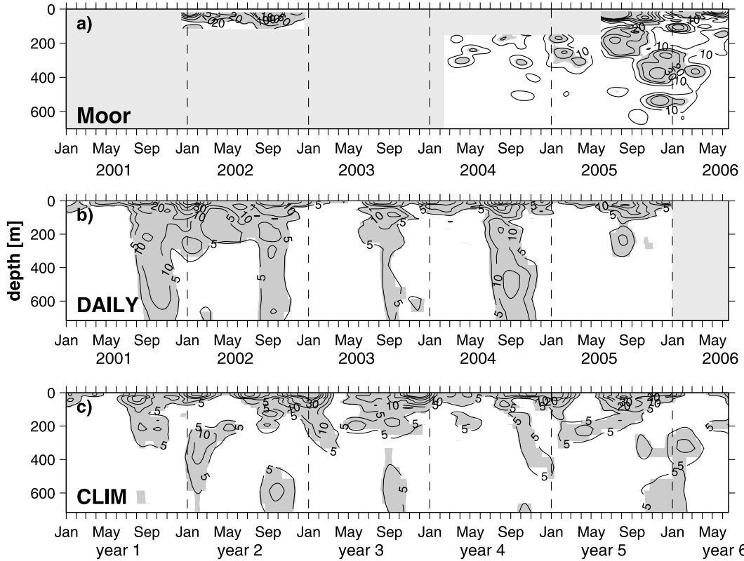
Figure 4. Normalized wavelet energy distributed with depths, averaged over a period range of 20 to 40 days derived from (a) current measurements, (b) the DAILY simulation, and (c) the CLIM simulation at 23^\circ\text{W} at the equator. Gaps in Figure 4a are due to missing measurements (light-gray shaded). Values above the 95% significance level are shaded dark gray and the black dashed line indicates the beginning of each year.
