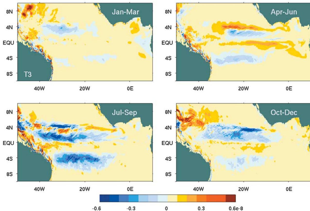
Figure 9. Seasonal maps of the baroclinic production term \overline{b'w'} ( \text{m}^2\text{s}^{-3} ), equation (1), derived from 6 years of the CLIM model simulation and averaged over the top 50 m. Negative sign denotes transfer from EPE into EKE.
