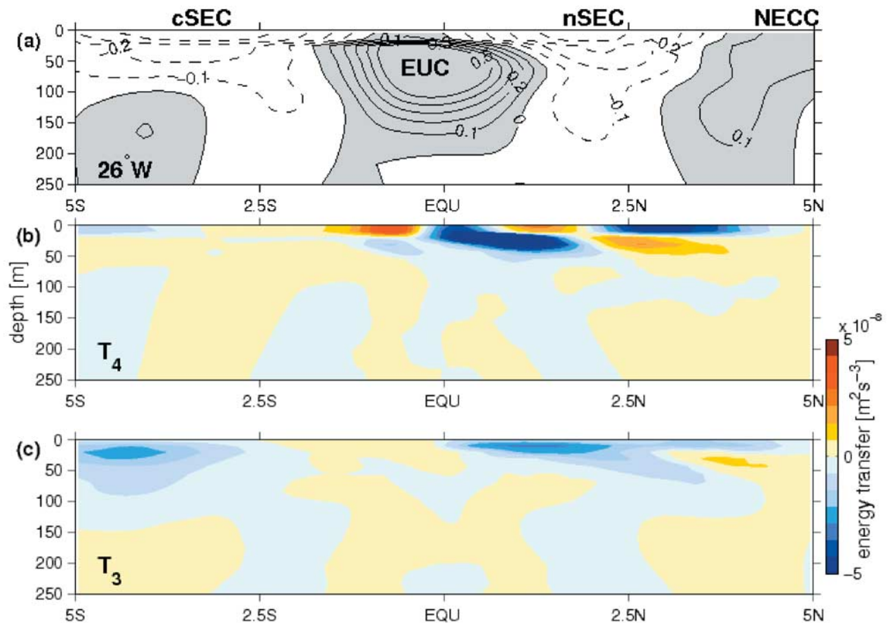
Figure 10. Results from 6 years of the CLIM simulation. (a) Mean zonal velocity along 26^{\circ}\text{W} , showing the central and northern South Equatorial Currents (cSEC and nSEC), the Equatorial Under Current (EUC) and the North Equatorial Counter Current (NECC). (b) Barotropic production rate \bar{S} averaged from 30^{\circ}\text{W} to 10^{\circ}\text{W} . Negative signs denote transfer into EKE. (c) Corresponding average of the baroclinic production term \bar{b'w'} . Negative signs denote transfer into EKE.
