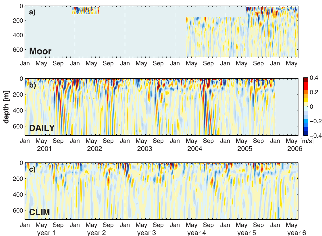
Figure 2. Meridional velocity at 23^{\circ}\text{W} at the equator from (a) 300 kHz WH-ADCP and 75 kHz Long Ranger ADCP, (b) the DAILY simulation (2001–2005), and (c) the CLIM simulation (6 years). Data are detided; small data gaps were interpolated. Dashed line marks the beginning of each year. Gaps in Figure 2a are due to missing measurements (light-gray shaded).
