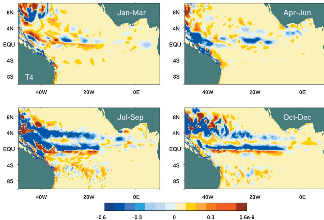
Figure 8. Seasonal maps of the barotropic instability production rate \bar{S} ( \text{m}^2\text{s}^{-3} ), equation (1), derived from 6 years of the CLIM model simulation and averaged over the top 50 m. Negative sign denotes transfer into the fluctuation.
