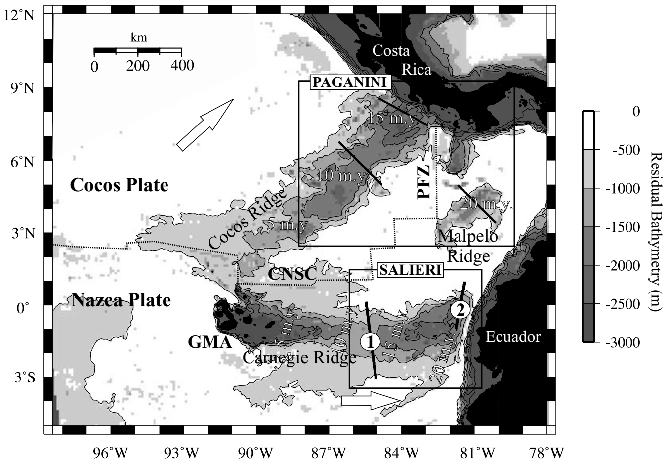
Figure 1. Location map of the study zone showing the residual bathymetry derived from the seafloor age (Mueller et al. 1996), based on the plate cooling model of Parsons & Sclater (1977) for ages smaller than 70 Myr ( d = 2500 + 350t^{1/2} ). Numbers show crustal ages of oceanic plates at 5 Ma intervals. Large arrows display plate motions relative to the stable South American craton (Trenkamp et al. 2002). Black lines show the location of all the wide-angle seismic profiles and numbers indicate the two profiles used in this work (profile 1, Western Carnegie; profile 2, Eastern Carnegie). Boxes outline the seismic experiments recently performed in Cocos, Malpelo and Carnegie (PAGANINI-1999; SALIERI-2001). CNSC, Cocos–Nazca Spreading Centre; GHS, Galápagos hotspot; PFZ, Panama fracture zone.
