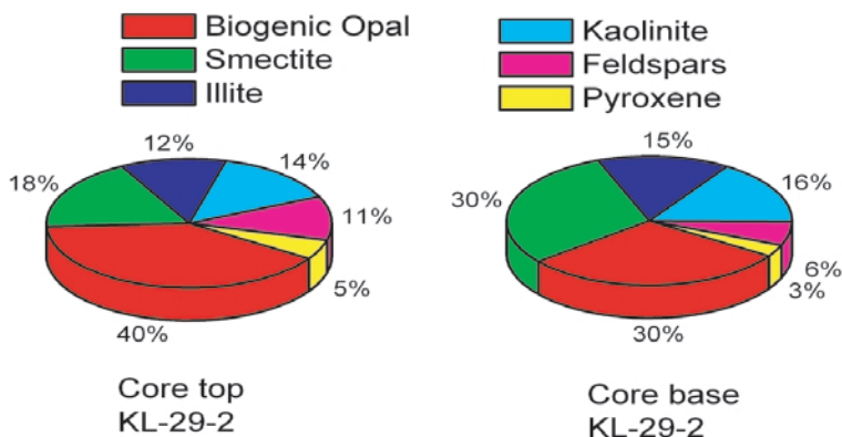
FIG. 1. Composition of surface sediments and core base sediments retrieved at the northern Sakhalin slope (KL-29-2).
