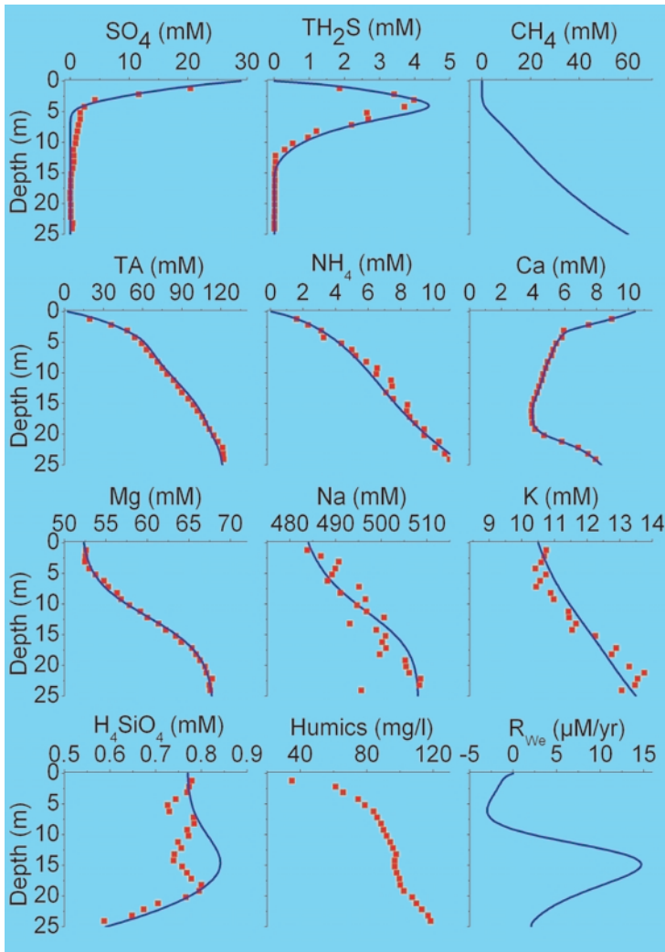
FIG. 2. Composition of pore fluids in sediments retrieved at the northern Sakhalin slope (KL-29-2). Red squares indicate data and blue curves represent the model results. TA is total alkalinity and R_{WE} gives the rate of CO_2 consumption via silicate weathering.
