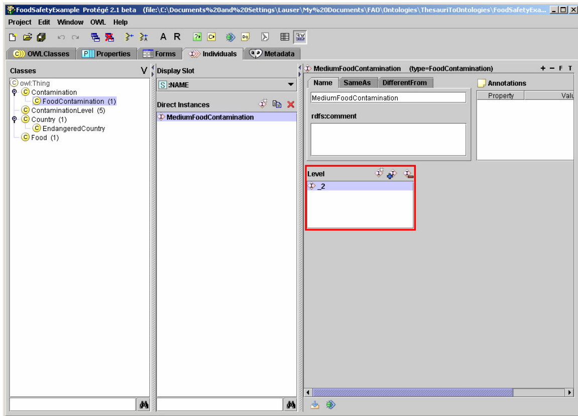
Figure 5: Enforcement of class level restrictions in OWL
