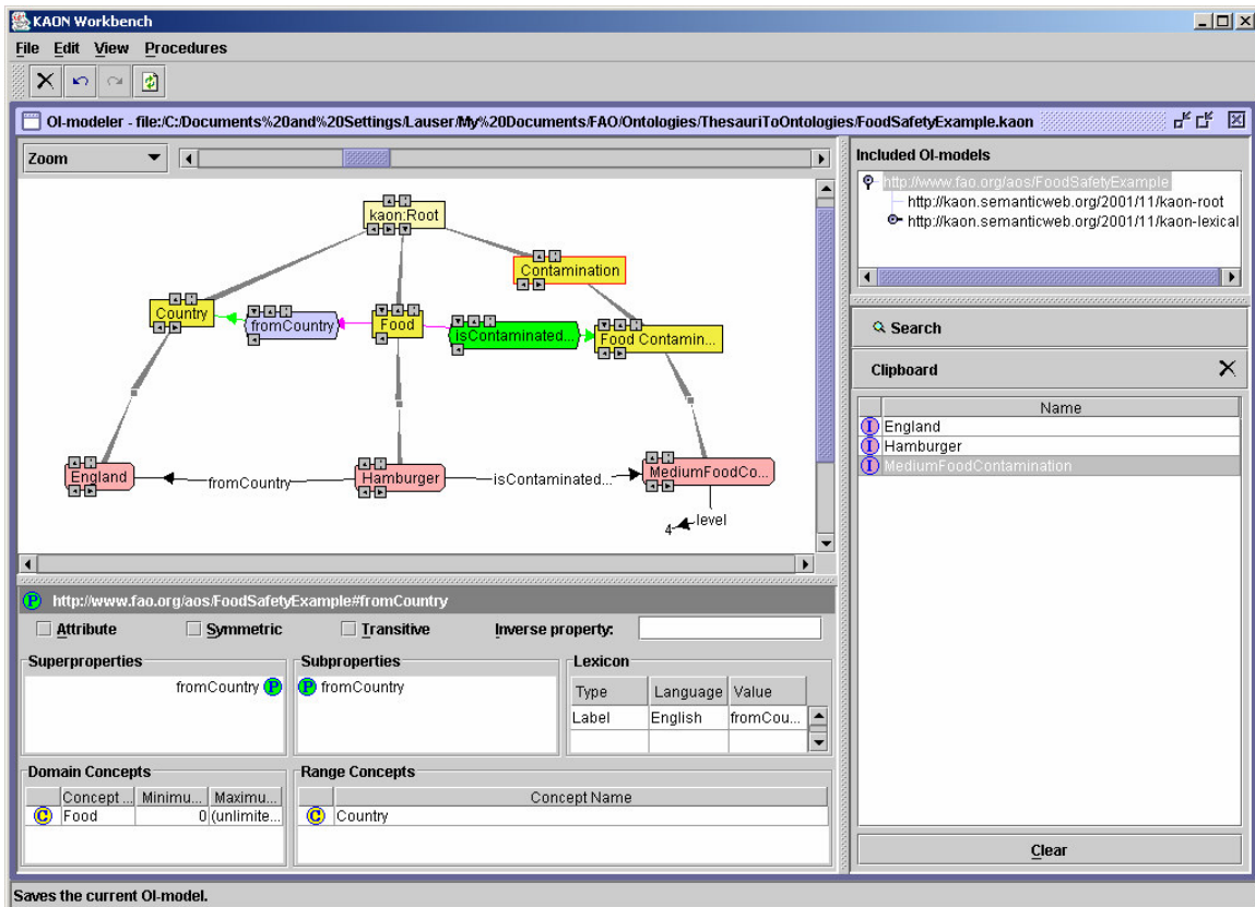
Figure 4: Instances in an RDFS ontology modelled in KAON
