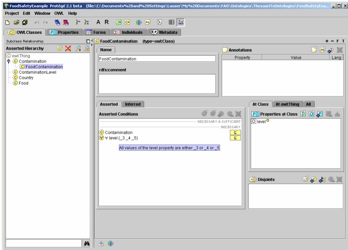
Figure 5: Modelling class level restrictions in OWL using Protégé
