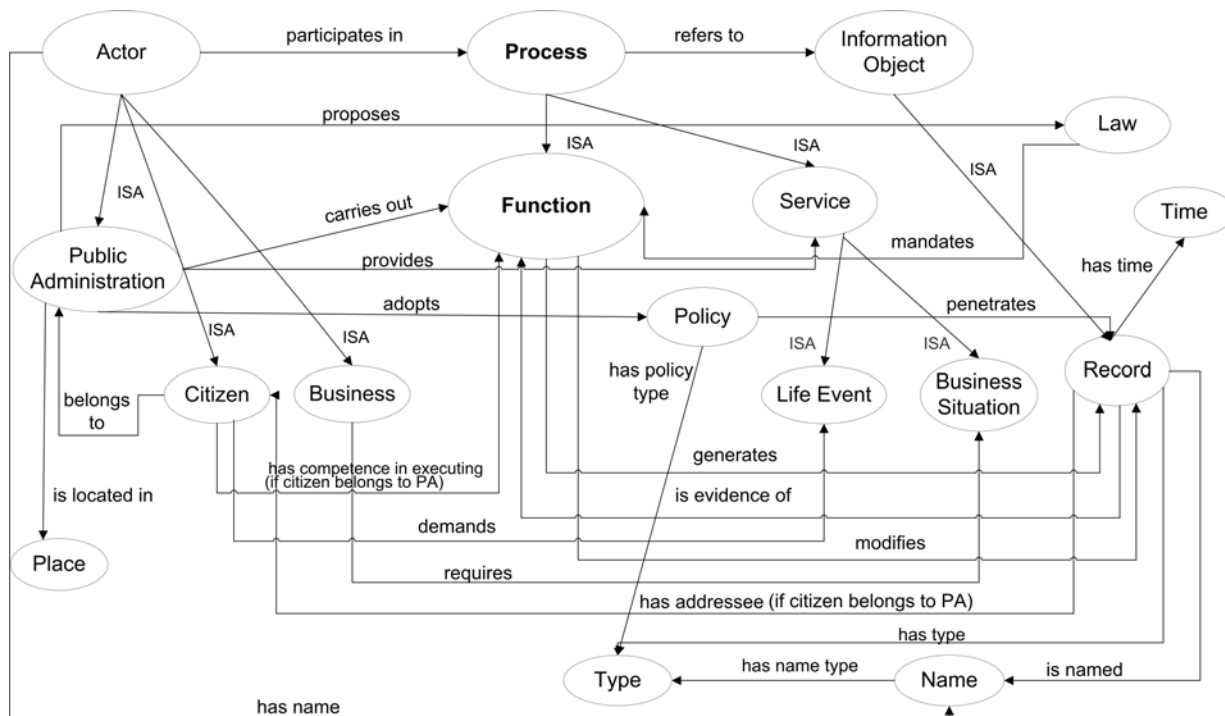
Figure 2. PSI ontology
