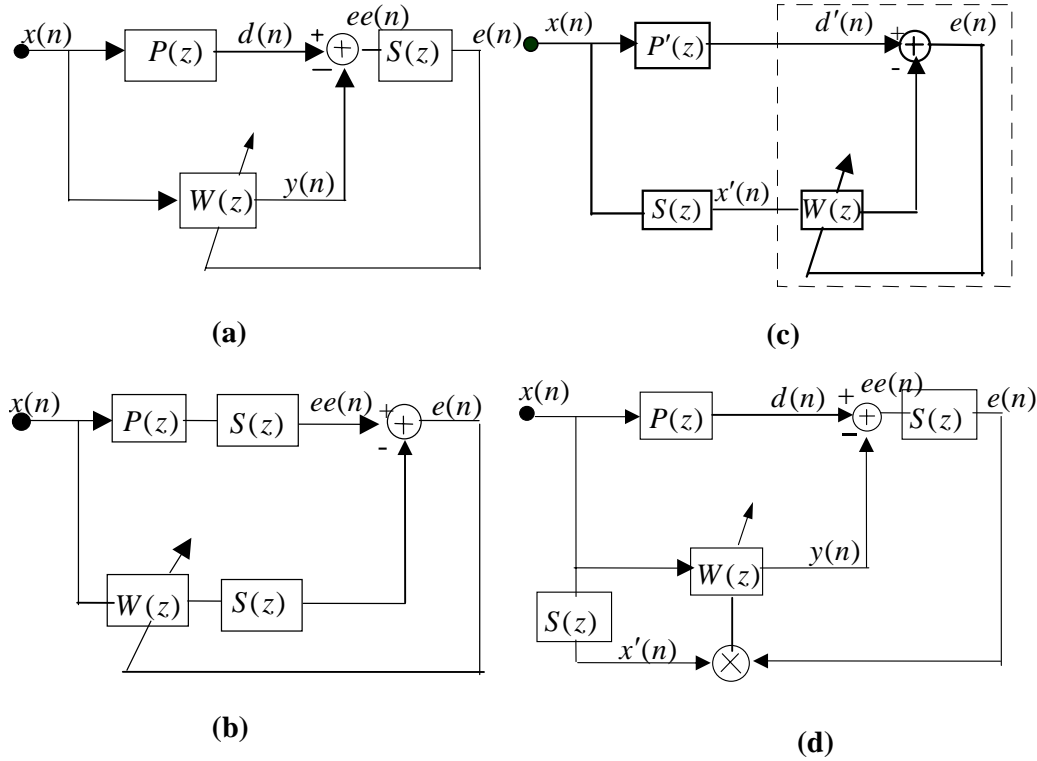
Fig.3 Development of FXLMS algorithm
