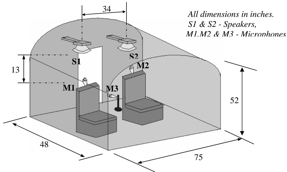
Fig. 8 Schematic of Multi-channel ANC in a cockpit mockup model
