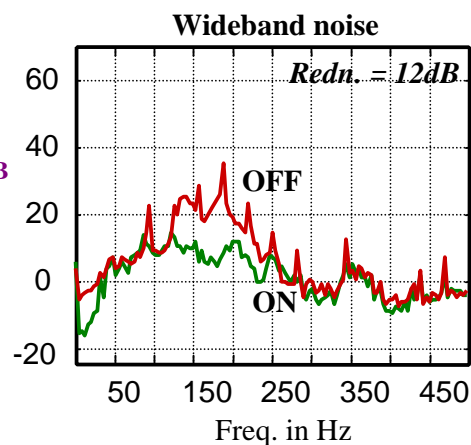
Fig. 6a Power spectral densities of signals with ANC OFF and ON microphones (to avoid feedback from secondary source to input microphone) are used for the in this study. The microphone is positioned sufficiently away 2' ( 4 times the
