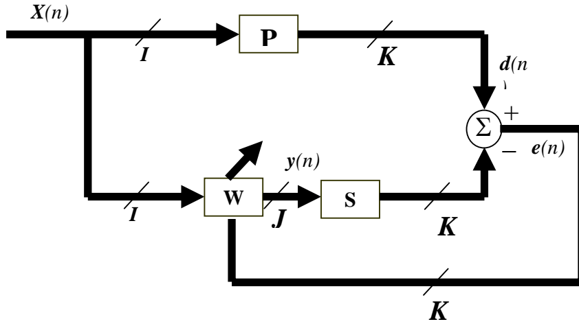
Fig. 5 Block schematic of multi-channel ANC system
