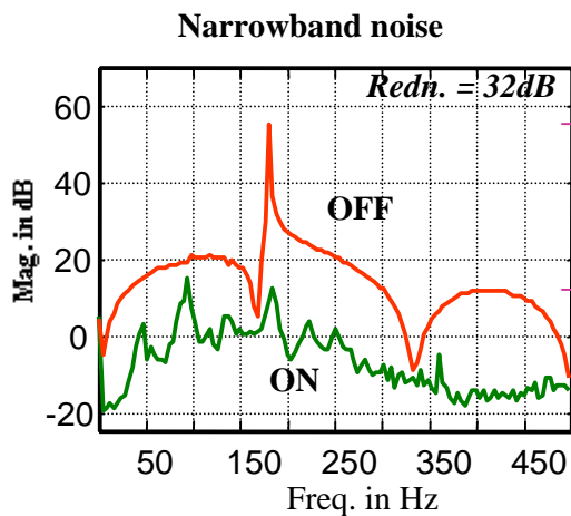
Fig. 6a Power spectral densities of signals with ANC OFF and ON microphones (to avoid feedback from secondary source to input microphone) are used for the in this study. The microphone is positioned sufficiently away 2' ( 4 times the
