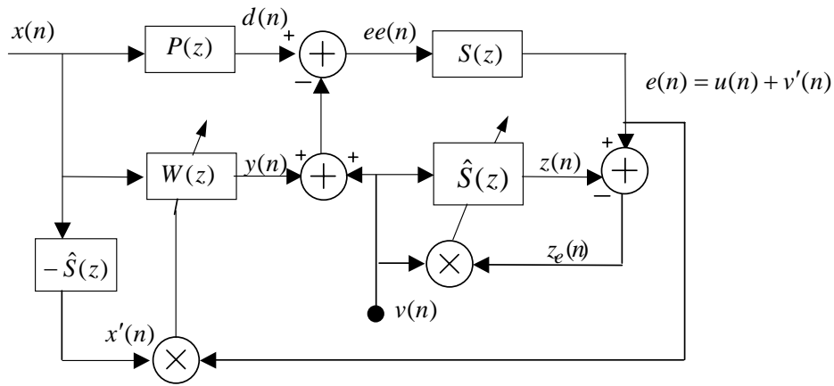
Fig. 4 FXLMS ANC with on-line secondary path modeling
