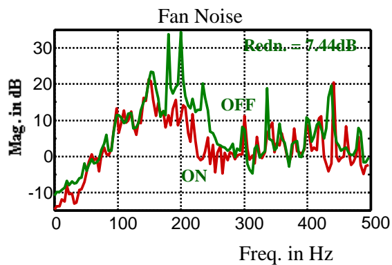
Fig. 7c Power Spectral density for noise at 80dB
