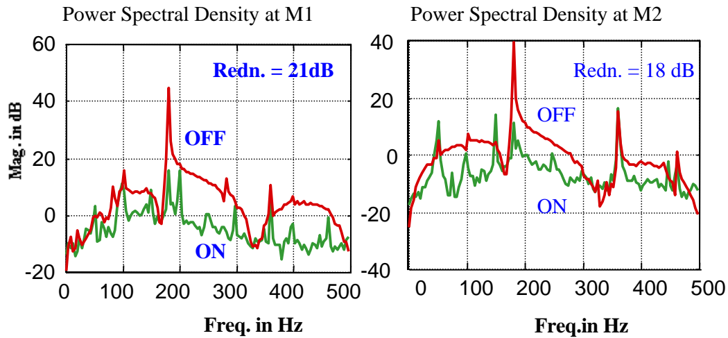
Fig. 9 Multichannel ANC for narrowband noise at 80dB
