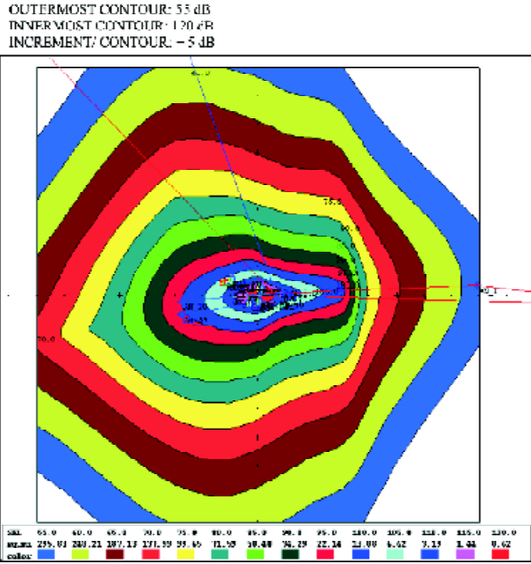
Figure 12. Individual aircraft (HPFA)-SEL noise contour.
