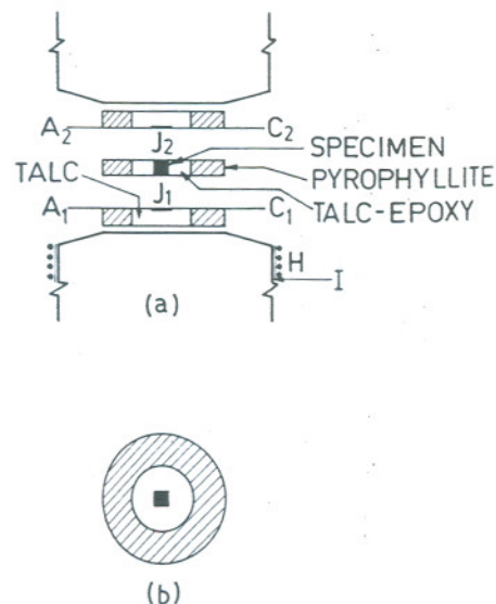
FIG. 1. (a) Schematic diagram of the high pressure cell. J_1, J_2 —thermojunctions. A_1, C_1, A_2, C_2 —thermocouples. H—heater, I—insulation. (b) Pyrophyllite gasket containing the sample set in talc epoxy.
