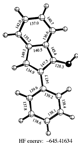
Fig. 2 HF/3-21G optimized structure of the ion obtained by the ring closure of protonated 2b and subsequent water elimination (bond lengths are in pm, HF energies are in hartrees)
