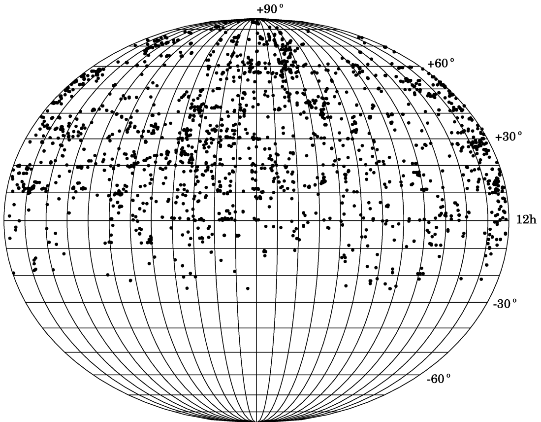
Fig. 1. All-sky distribution of the KON060 plate centers.
