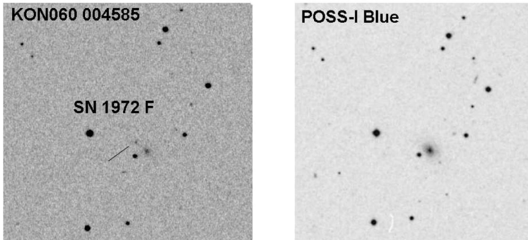
Fig. 4. Part of KON060 004585 plate with the discovered SN 1972F and the same region from POSS-I Blue.
