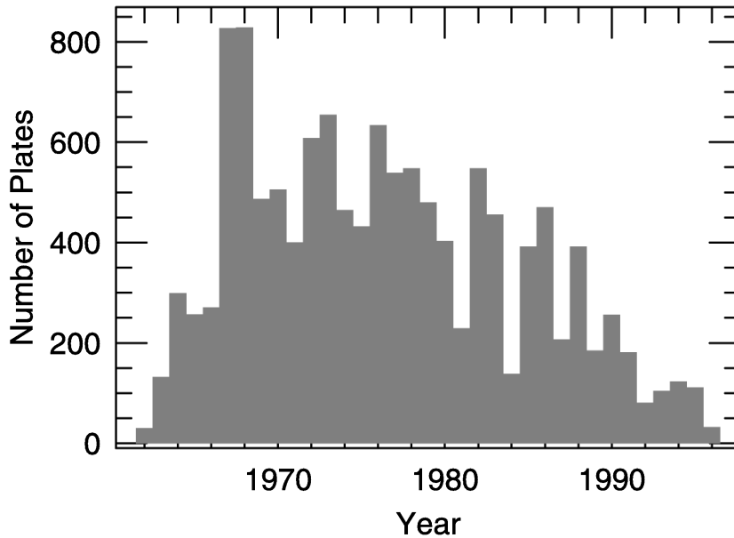
Fig. 2. Time distribution of amount of the Konkoly Schmidt telescope plates.
