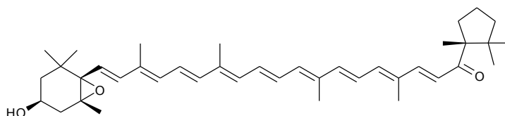
3'-Deoxycapsanthin-5,6-epoxide ( 6 )
