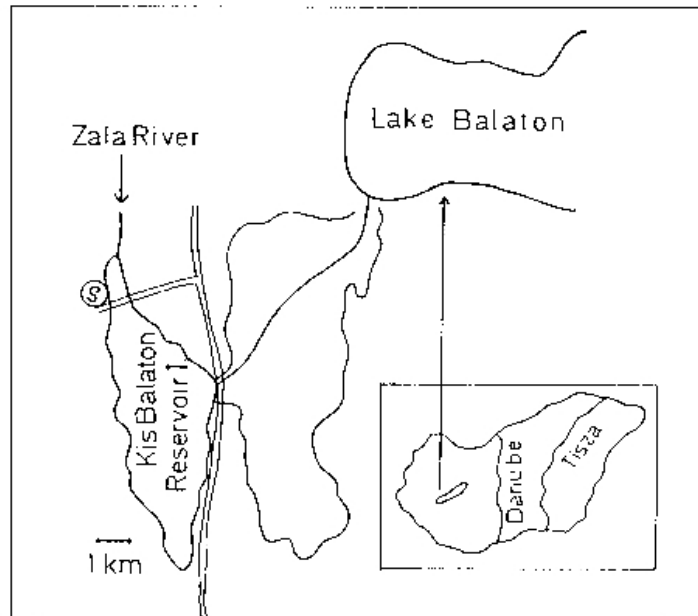
Fig. 1. Map of Kis-Balaton Reservoir, S – sampling station
