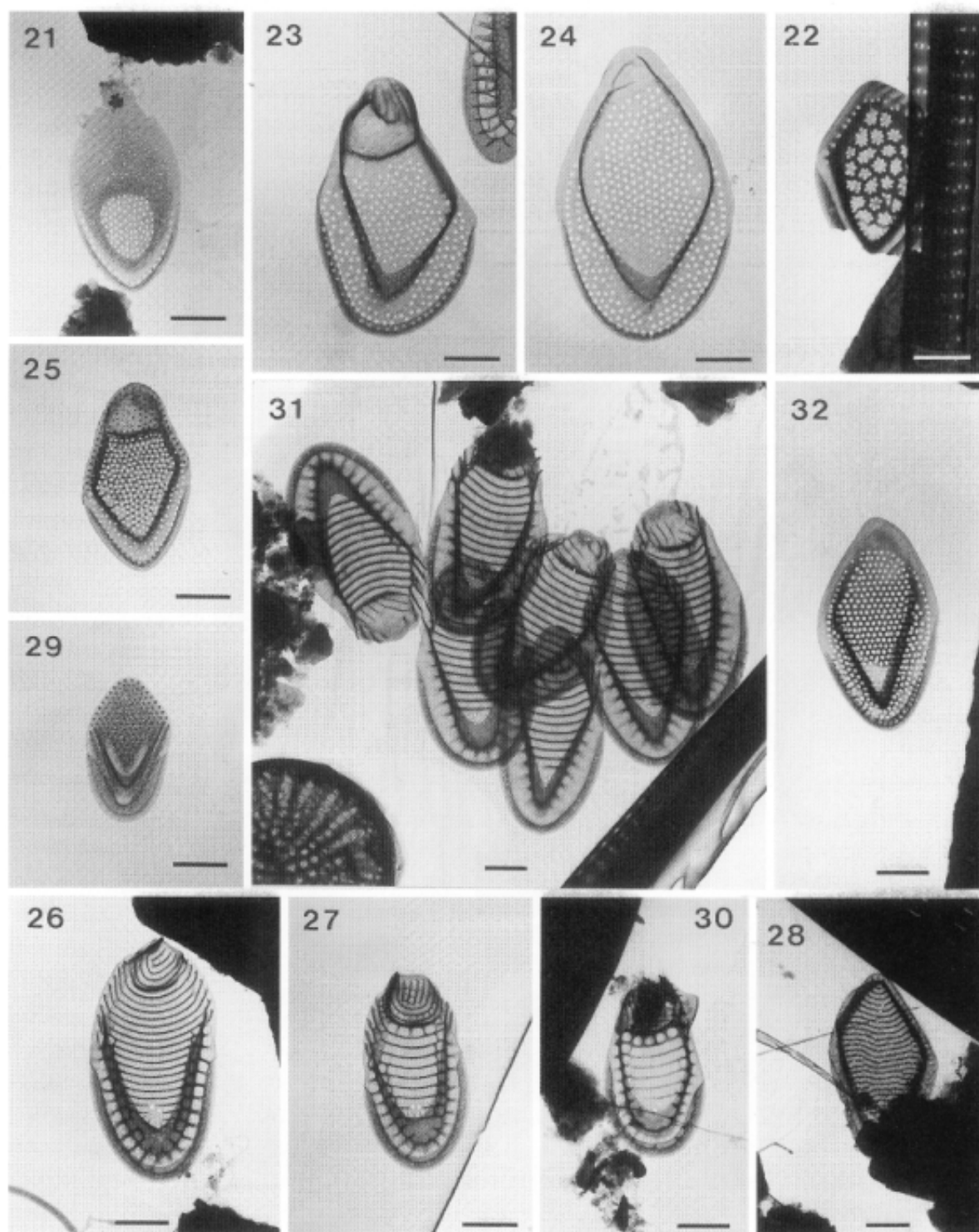
Fig. 2. – continued (21–32). 21- Mallomonas akrokomos , body scale; 22- Mallomonas alata , body scale; 23- Mallomonas alpina , dome-bearing apical scale, 24- Mallomonas alpina , domeless body scale; 25- Mallomonas annulata , dome-bearing body scale; 26, 27- Mallomonas cratis , two different types of scales; 28- Mallomonas schwemmlei , body scale; 29- Mallomonas parvula , body scale; 30- Mallomonas pseudocratis , body scale; 31- Mallomonas striata , body scales; 32- Mallomonas tonsurata , domeless body scale. The scale-bars indicate 1 \mu m.
