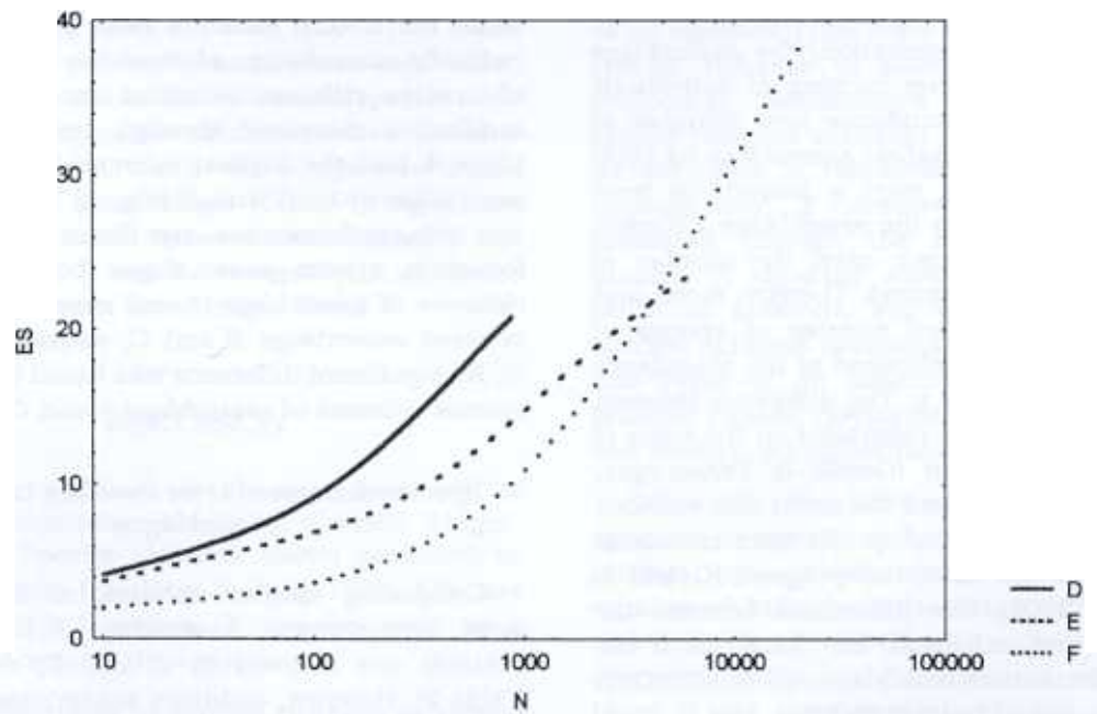
Figure 2. The comparison of species richness of river assemblages (D, E and F) using rarefaction
