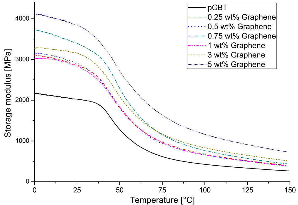
Figure 4 Storage modulus vs. temperature curves of pCBT and pCBT nanocomposites containing different amounts of graphene
