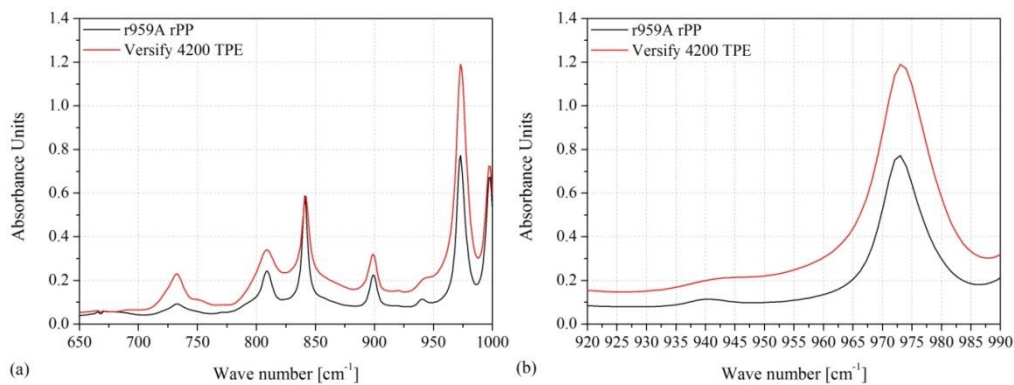
Figure 1 FTIR spectra of the TPE matrix (Versify 4200) and the conventional rPP (r959A) (a) and the related sections between 920-990 \text{cm}^{-1} (b)
