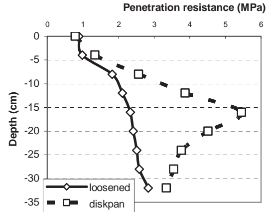
Figure 1. Penetration resistance curves of a loosened and a diskpan compacted soil
