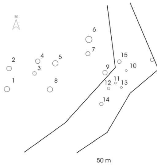
Fig. 4. Structure of the mature cypress forest. Circles are proportional to trunk diameter at ground level. Heavy lines indicate work walls in July 2007. Fifteen trunks were excavated and measured. The sixteenth one in the far right was made unavailable by quicksand. Map courtesy of Bükkábrány Mine, Ltd.
