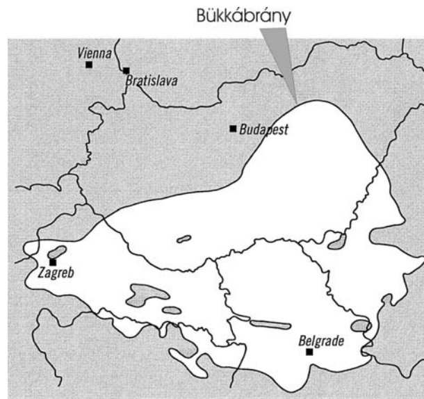
Fig. 2. Location of Bükkábrány at the northern margin of Lake Pannon – white, surrounded by land, shaded – in the Late Miocene (8 Ma palaeogeography map: MAGYAR et al. 1999).
