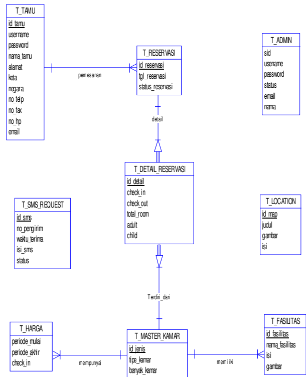
Gambar 4. Model Conceptual Database
