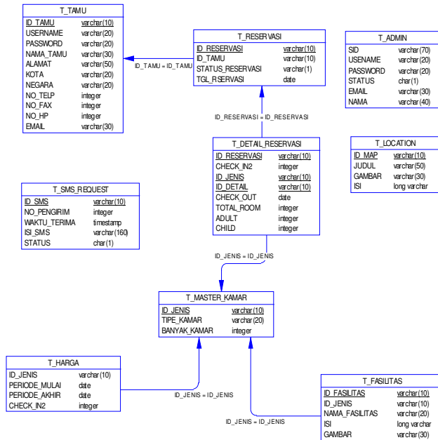
Gambar 5. Model Physical Database
