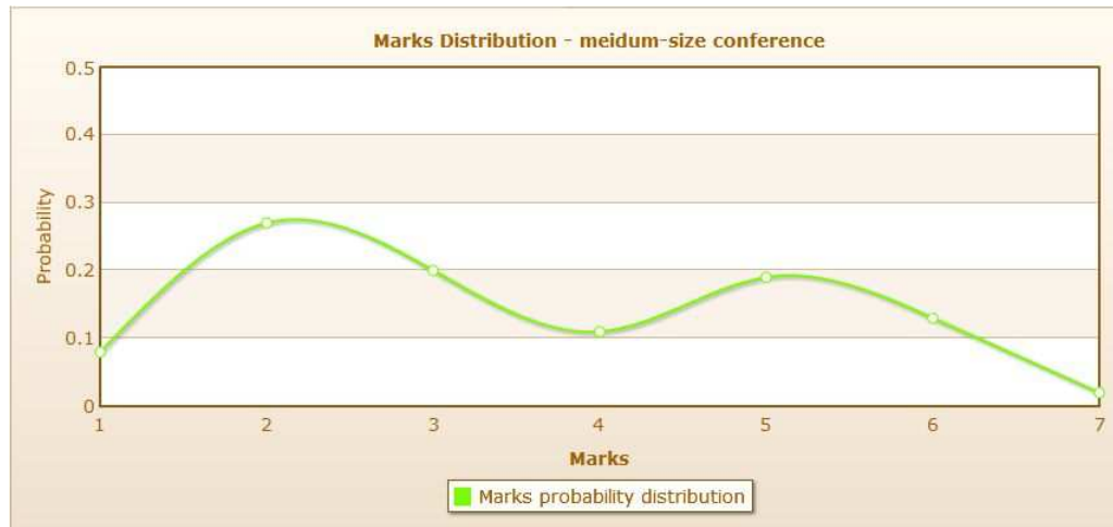
Fig. 16: Marks distribution
