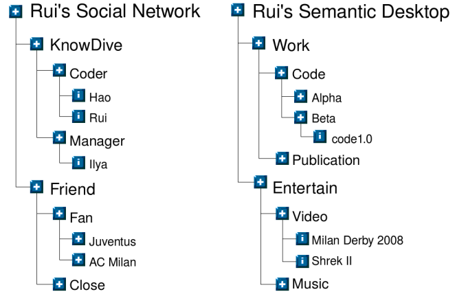
Fig. 2. SUBJECT and OBJECT Hierarchies.
