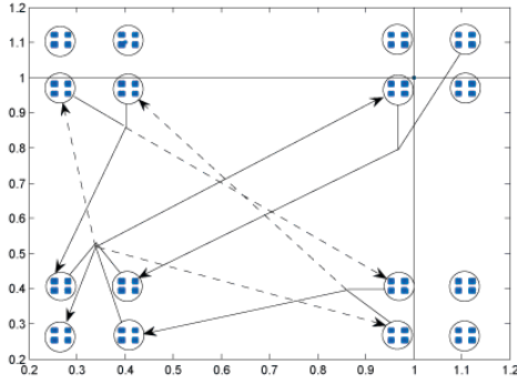
Fig. 1. Attractor of system (12)
