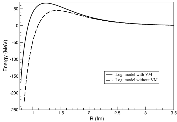
Figure 3.9: Total energy of the soliton at mean-field level in the logarithmic model without vector mesons (dashed line) and with vector mesons (solid line). The parameter values are: m_\sigma = 1200 MeV, g_\pi = 5 , g_\omega = 12 and g_\rho = 4 .
