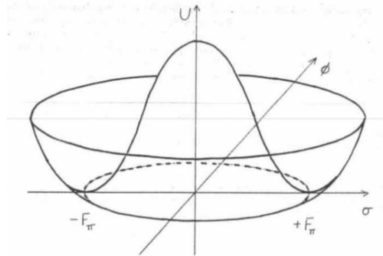
Figure 1.5: The Mexican hat potential for the meson fields in the Linear- \sigma model.
