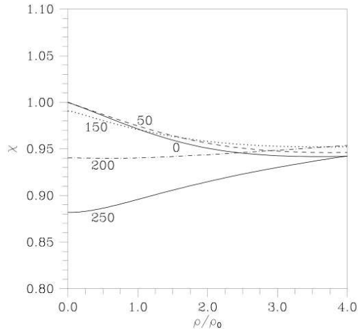
Figure 2.1: The glueball mean-field ratio \chi as a function of density for various temperatures in MeV.
