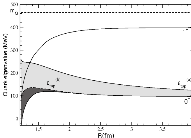
Figure 3.7: Lower panel: quark eigenvalue as a function of the cell radius R , in the model without vector mesons. The shaded areas represent the band as estimated in eq.(3.9) and in eq. (3.11). The quark mass in vacuum, here 465 MeV, is indicated by the dashed line.
