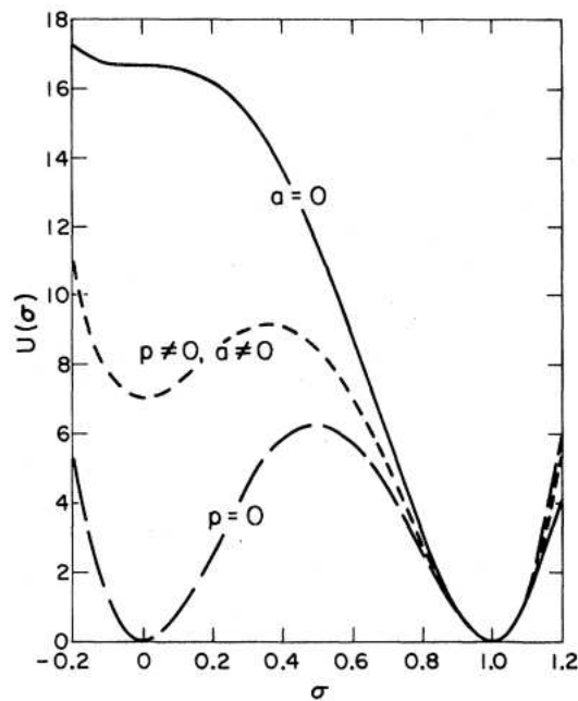
Figure 1.1: Typical forms for the potential U(\sigma) in the soliton bag model.
