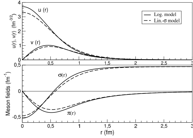
Figure 2.4: Upper panel: Dirac components in the CDM (solid line) and in the Linear \sigma -model (dashed line) without vector mesons. Lower panel: chiral fields in the CDM (solid line) and in the Linear \sigma -model (dashed line) without vector mesons.
