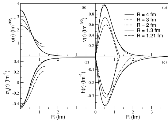
Figure 3.1: Upper (panel (a)) and lower (panel (b)) components of the Dirac spinor, \sigma (panel (c)) and pion (panel (d)) fields for different values of the cell radius R in the model without vector mesons.
