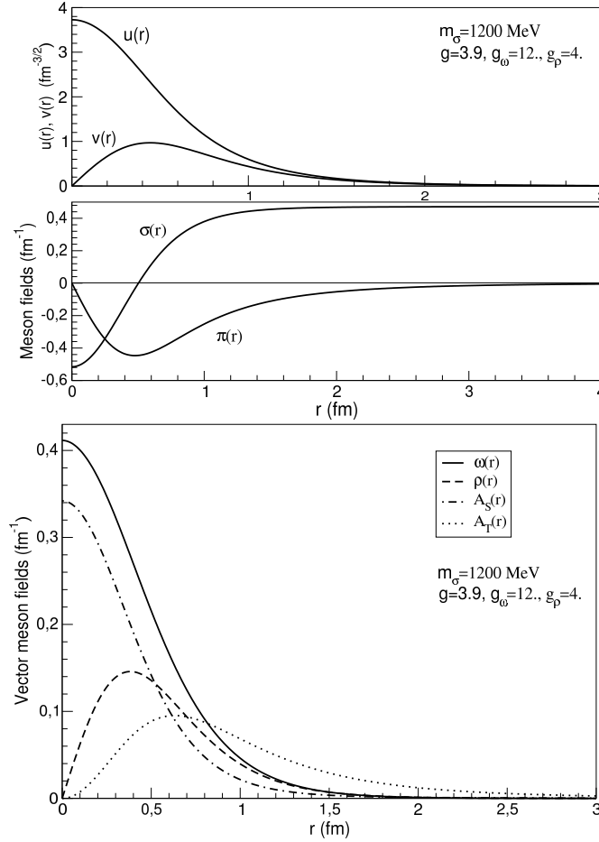
Figure 2.5: Left panel: Dirac components (upper panel) and chiral fields (lower panel) in the CDM with vector mesons for set I. Right panel: vector mesons profiles in the CDM for set I.
