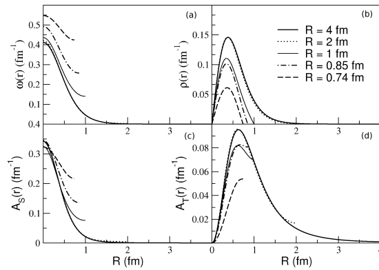
Figure 3.2: Vector mesons fields, as functions of the cell radius R . In (a) we plot the \omega field, in (b) the \rho field, in (c) the A_S field and in (d) the A_T field.
