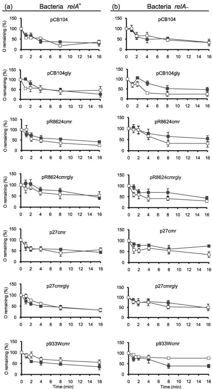
Fig. 5. Stability of the O protein in reIA + (left panels) and reIA - (right panels) E. coli cells bearing the plasmids indicated in each panel. The bacteria were either starved for isoleucine (open symbols) or not starved (closed symbols). Results shown are mean \pm SD from three experiments.
