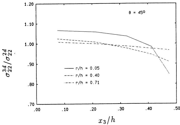
Figure 4.17: Through-thickness variation of a) the plane-strain constraint, b) \sigma_{11} and c) \sigma_{22} .
