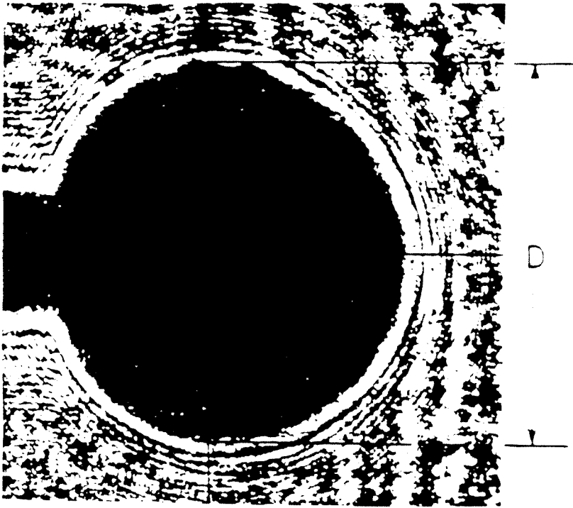
Figure 2.2: Representative caustic pattern from a statically loaded fracture specimen.
