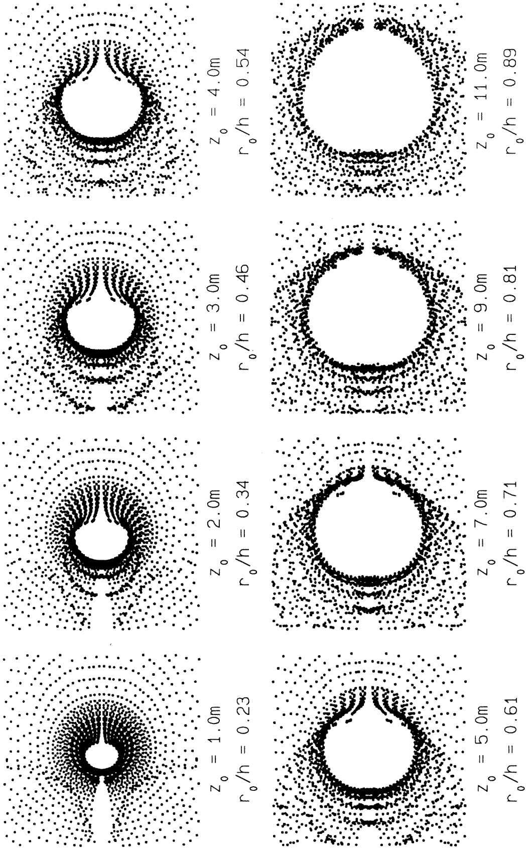
Figure 4.11a: Simulated caustics from the computed three dimensional free surface u_3 -displacements.
