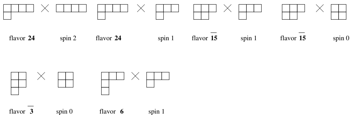
Figure 3.6: Young tableaux showing the flavor SU(3) \times spin SU(2) decomposition of the positive-parity \bar{q}Qqqq pentaquarks. The two representations in the lower row contain no exotic states.
