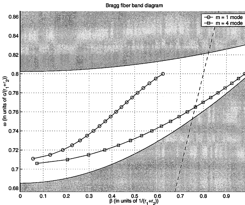
Fig. 14. Dispersion diagram based on asymptotic calculations. Just as in Fig. 10, only the TM-like bands with the lowest radial number are plotted. Boundary conditions are matched at the 50th cladding layer. Fiber parameters are given in the caption of Fig. 10. Note that the m = 4 band was missing in Fig. 10.
