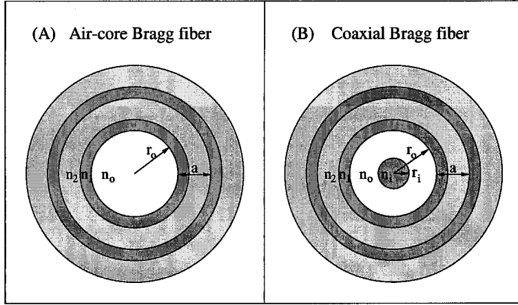
Fig. 1. Air-core and coaxial Bragg fiber cross sections. (A) Air-core Bragg waveguide, and (B) Coaxial Bragg waveguide. Cladding layer 1 has an index of refraction n_1 = 4.6 and a thickness d_1 = 0.333a (not shown), whereas layer 2 an index of refraction n_2 = 1.6 and a thickness d_2 = 0.667a (not shown), where a = d_1 + d_2 is the period of the cladding. The white region in the core is assumed to be filled with air, with an index of refraction n_o = 1 . Three parameters are subject to change in this study: n_i , the index of the refraction of the inner core in (B); r_i , the radius of the inner core in (B); and r_o , the outer core radius in both (A) and (B). Note that an air-core Bragg fiber can be thought as a coaxial Bragg fiber with r_i = 0 .
