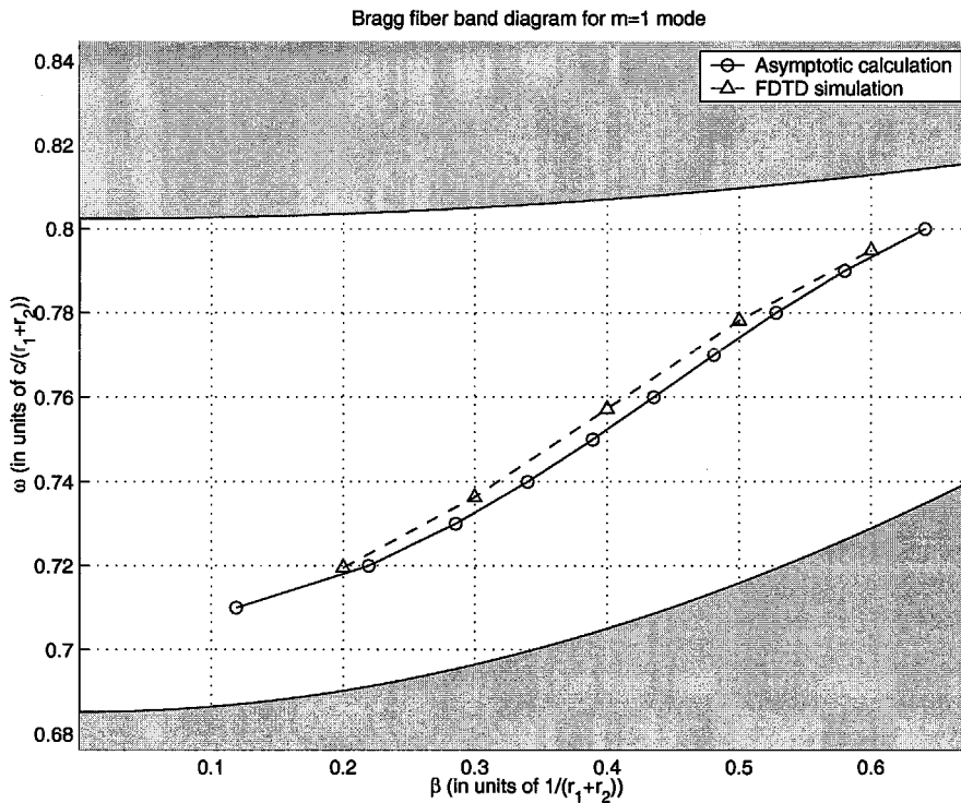
Fig. 12. Dispersion diagram for the m = 1 mode. The asymptotic curve is copied from Fig. 10 and the FDTD structure is defined with 12 cladding pairs.
