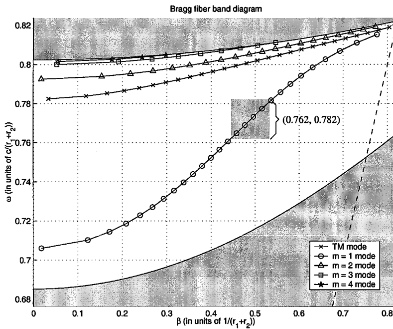
Fig. 10. Dispersion diagram based on asymptotic calculations. Only the TM and TM-like modes with the lowest radial number are plotted, as all other modes have been “pushed” out of the bandgap. The TM band structure of the corresponding Bragg stack serves as the background and the dotted line shown is the light line. Boundary conditions are matched at the air core boundary. The following fiber parameters are used: n_1 = 4.6 , n_2 = 1.5 , r_1 = 10 , r_2 = 2 , and r_{core} = 30 , all in normalized units. Note in the frequency window (0.762, 0.782) the m = 1 band not only exhibits single-mode behavior but also possesses negative dispersion values.
