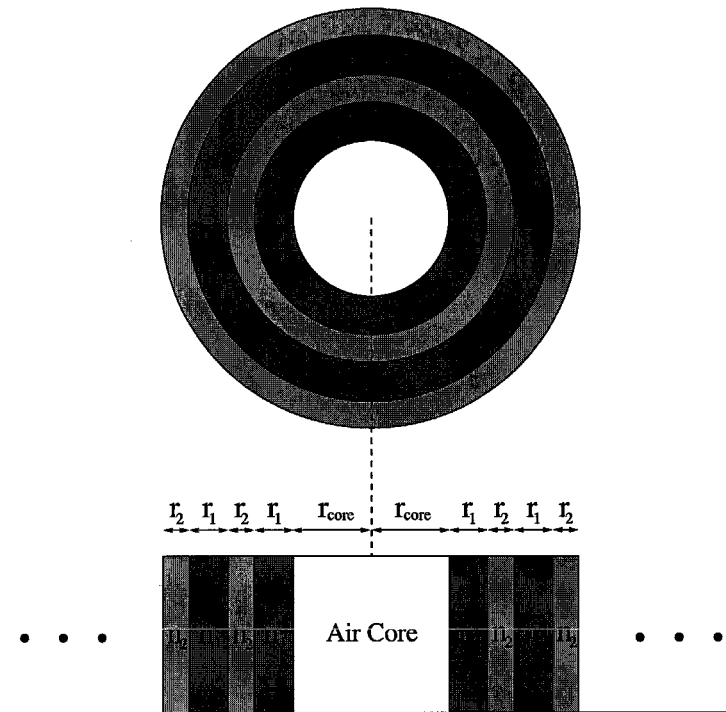
Fig. 9. Schematic of an air-core Bragg fiber. The fiber cladding consists of alternating layers of dielectric media with high and low refractive indices.
