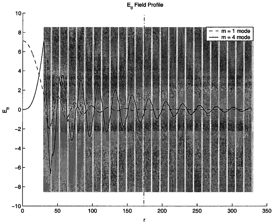
Fig. 15. The radial profile of the E_\theta field. The white area is the fiber core and the shaded layers represent the cladding layers. All fiber parameters are given in the caption of Fig. 10. The vertical dashed line shows the boundary of a fiber structure with 12 cladding pairs, used in the FDTD simulations in Sec. 3.3. The frequency of the mode is \omega = 0.77(c/(r_1+r_2)) , the chosen normalized operating frequency.
