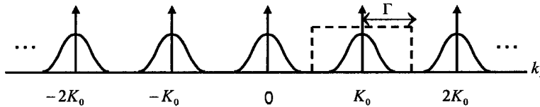
Fig. 19. Fourier spectrum of \Delta(\tilde{n}^2) . Valid when a_m 's and b_m 's are slowly varying. Note only the two resonant components at K_0 and -K_0 can provide coupling between the forward and backward propagating waves.
