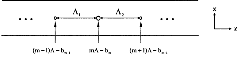
Fig. 20. Local period at the m th air hole. The local period at a given air hole is defined to be the average of the distances to the two adjacent air holes, i.e., (\Lambda_1 + \Lambda_2)/2 .
