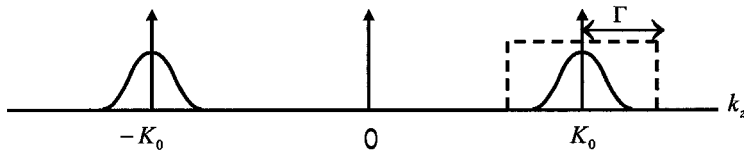
Fig. 18. Fourier spectrum of \Delta(n^2) . Valid when \Delta n(z) and \theta(z) are slowly varying.
