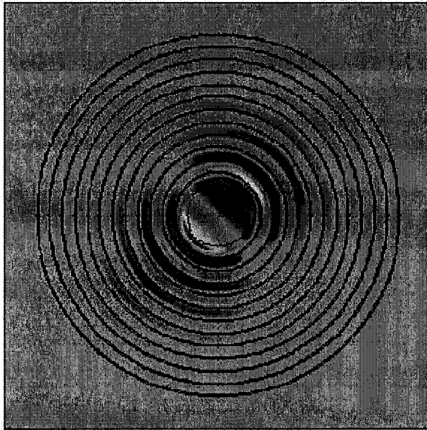
Fig. 13. H_z field distribution of the m = 1 mode. The field is obtained by FDTD calculations. The parameters of the Bragg fiber are given in the caption of Fig. 10. The Bragg cladding consists of 12 cladding pairs and the whole fiber is immersed in air. The angular frequency and propagation constant of this mode are \omega = 0.777(c/(r_1 + r_2)) and \beta = 0.5(1/(r_1 + r_2)) , respectively.
