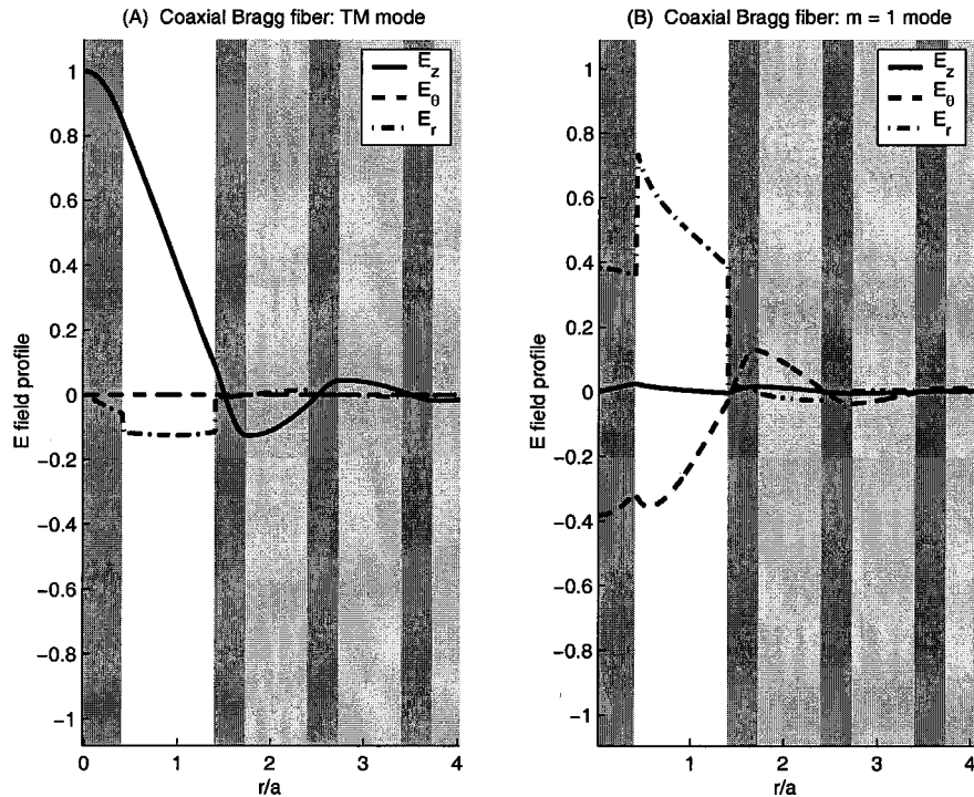
Fig. 5. \vec{E} field profiles for n_i = 1.45 , r_i = 0.4a , and r_o = 1.4a . The propagation constant \beta = 0.05(2\pi/a) for both plots and the eigen frequency \omega are found to be: (A) \omega = 0.2267(2\pi c/a) , (B) \omega = 0.1966(2\pi c/a) . Note that in (B) the jump discontinuity for E_r at the core boundary is not as sharp as that of Fig. 3(D).
