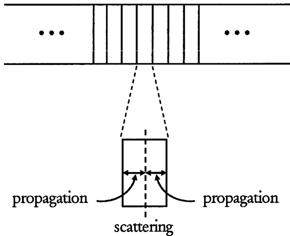
Fig. 16. Layer peeling algorithm. As proposed in [27], the fiber is divided into discrete layers of constant coupling coefficients. The transfer matrix of each layer is then approximated by an instantaneous scattering matrix sandwiched between two identical propagation matrices
