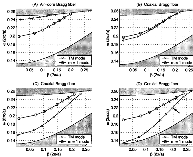
Fig. 2. Dispersion diagrams for n_i = 4.6 and r_o = 1.4a . r_i is varied as follows: (A) r_i = 0 (air-core Bragg fiber), (B) r_i = 0.133a , (C) r_i = 0.2a , and (D) r_i = 0.267a . Note in (D) the TM mode exhibits single-mode behaviour in the lower half of the bandgap, which does not include the zero-dispersion point identified by the arrow.
