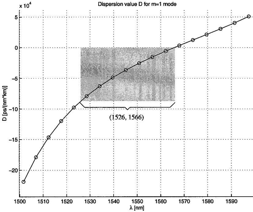
Fig. 11. Dispersion value D for the m = 1 band. Curve is plotted based on asymptotic calculations. The second derivative \partial^2\beta/\partial\omega^2 is calculated by a direct differential method (i.e., no curve fitting). Fiber structure and boundary matching surface follow those of Fig. 10. Shaded area (1526, 1566) is made to match the frequency window (0.762, 0.782), also in Fig. 10, by choosing the normalized operating frequency to be 0.77(c/(r_1 + r_2)) , which translates to 1.55\mu\text{m} in MKS units. Note at \lambda = 1.55\mu\text{m} , dispersion value D \approx -25,000\text{ps}/(\text{nm}\cdot\text{km}) .
