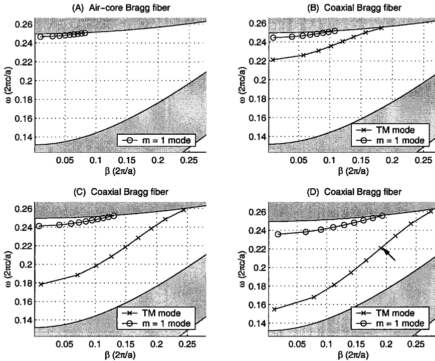
Fig. 6. Dispersion diagrams for n_i = 4.6 and r_o = 0.867a . r_i is varied as follows: (A) r_i = 0 (air-core Bragg fiber), (B) r_i = 0.133a , (C) r_i = 0.2a , and (D) r_i = 0.267a . Note that in (D) the TM mode exhibits single-mode behaviour almost all the way through the bandgap, with the zero-dispersion point (identified by the arrow) falling inside the single-mode frequency range.
