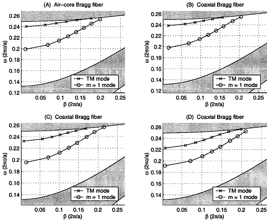
Fig. 4. Dispersion diagrams for n_i = 1.45 and r_o = 1.4a . r_i is varied as follows: (A) r_i = 0 (air-core Bragg fiber), (B) r_i = 0.133a , (C) r_i = 0.267a , and (D) r_i = 0.4a . Note the downward shifts of the two bands are small compared to those of Fig. 2.
