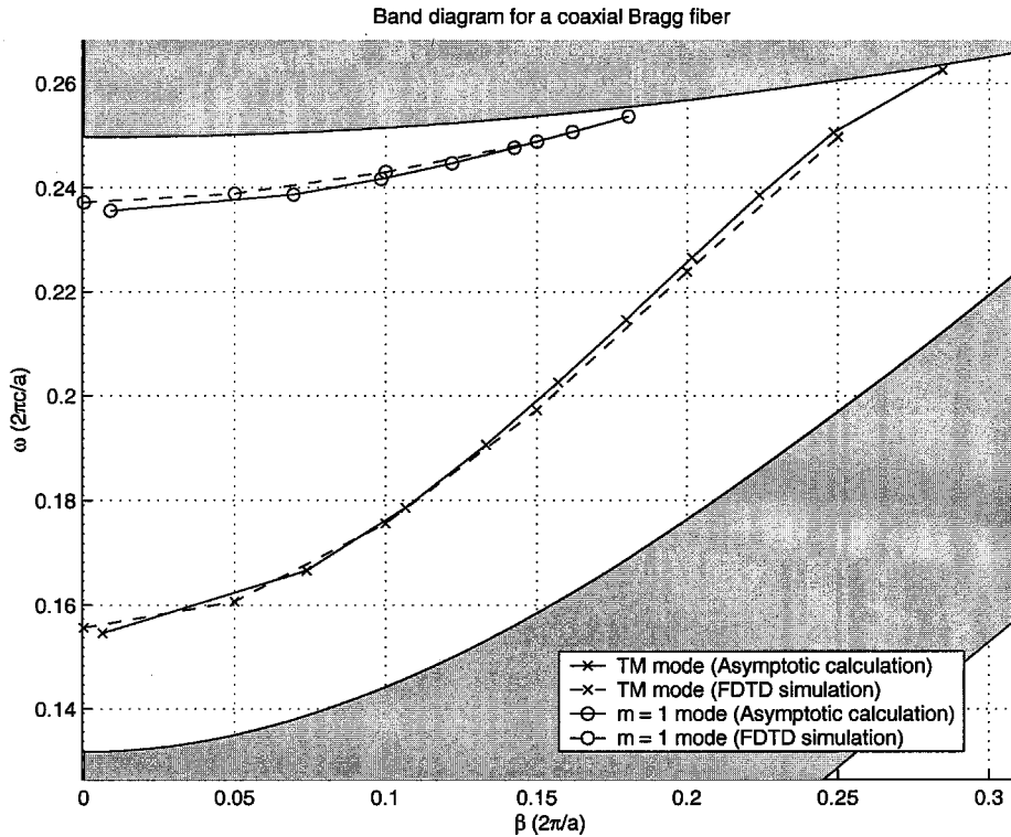
Fig. 7. Asymptotic calculation vs. FDTD simulation. Coaxial fiber band diagram for n_i = 4.6 , r_i = 0.267a , and r_o = 0.867a . The asymptotic curves are copied from Fig. 6(D) and the FDTD structure is defined with 5 cladding pairs.
