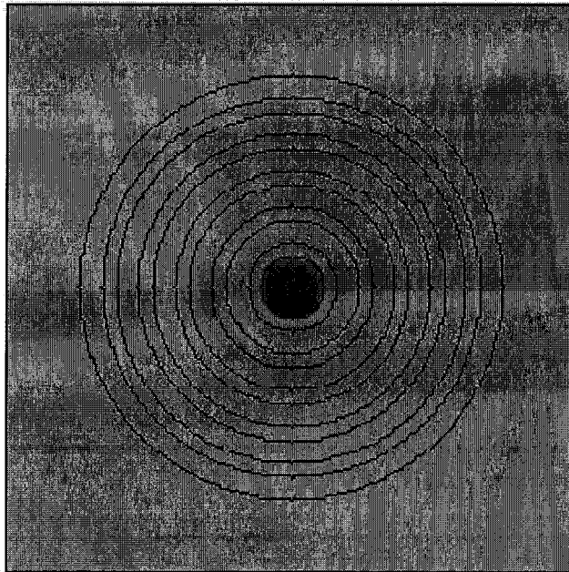
Fig. 8. E_z field distribution of the TM mode. The field is obtained by FDTD calculations. The parameters of the Bragg fiber are given in the caption of Fig. 1 with n_i = 4.6 , r_i = 0.267a , and r_o = 0.867a . The Bragg cladding consists of 5 cladding pairs and the whole fiber is immersed in air. The frequency and propagation constant of the mode are \omega = 0.2238(2\pi c/a) and \beta = 0.2(2\pi/a) , respectively.
